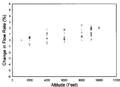
FIGURE 3. Change in flow rate versus altitude at a 2.0 L/min set point.
