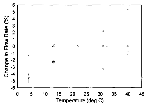
FIGURE 12. Change in flow rate versus temperature at a 2.0 L/min set point.
