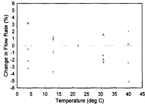
FIGURE 11. Change in flow rate versus temperature at a 1.0 L/min set point.
