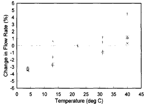
FIGURE 13. Change in flow rate versus temperature at a 3.0 L/min set point.
