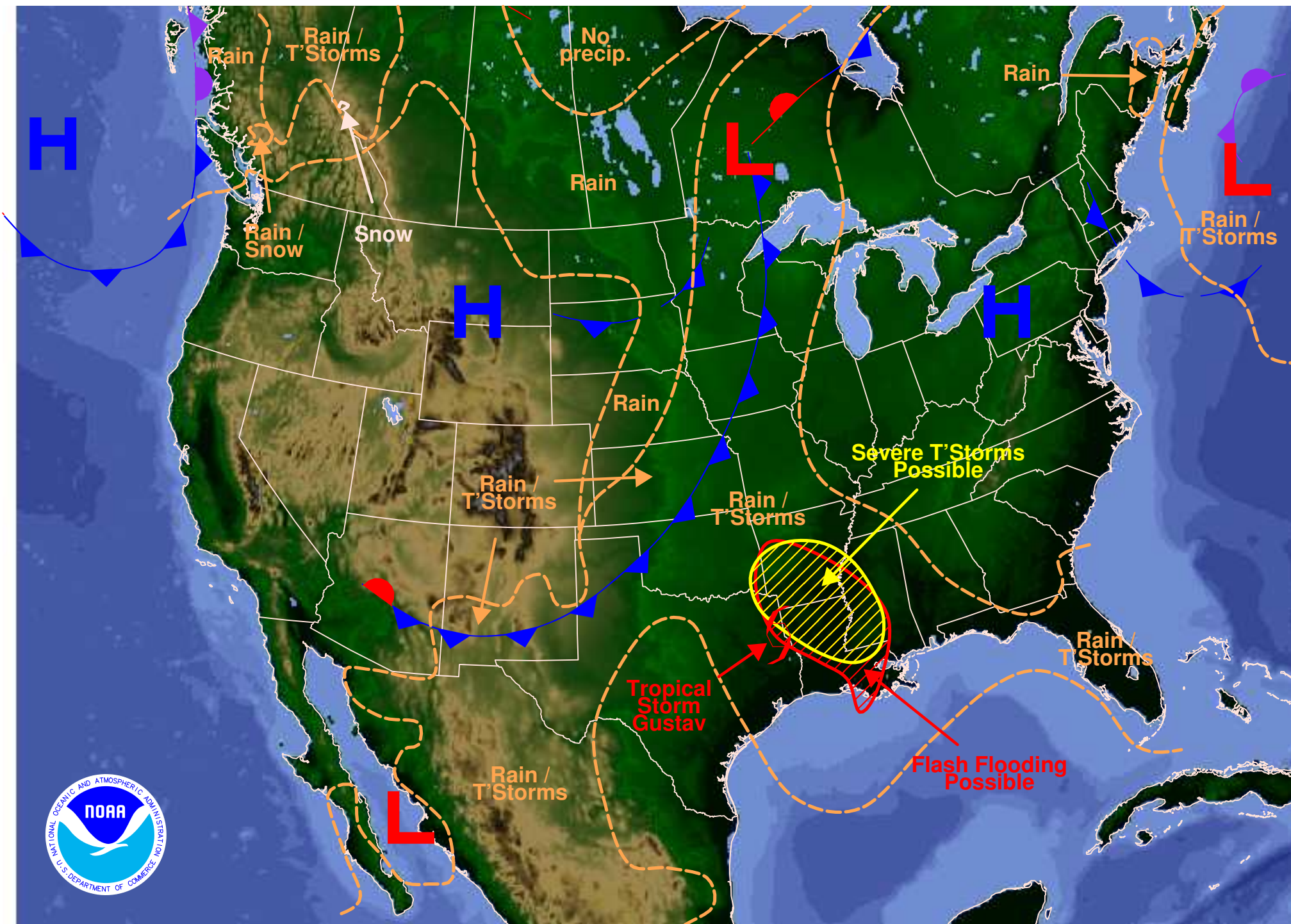
Weather Forecast for Tuesday, September 02, 2008 DOC/NOAA/NWS/NCEP/Hydrometeorological Prediction Center Prepared by Kong based on HPC, SPC, and TPC forecasts.
