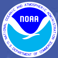
Weather Forecast for Tuesday, September 02, 2008 DOC/NOAA/NWS/NCEP/Hydrometeorological Prediction Center Prepared by Kong based on HPC, SPC, and TPC forecasts.
