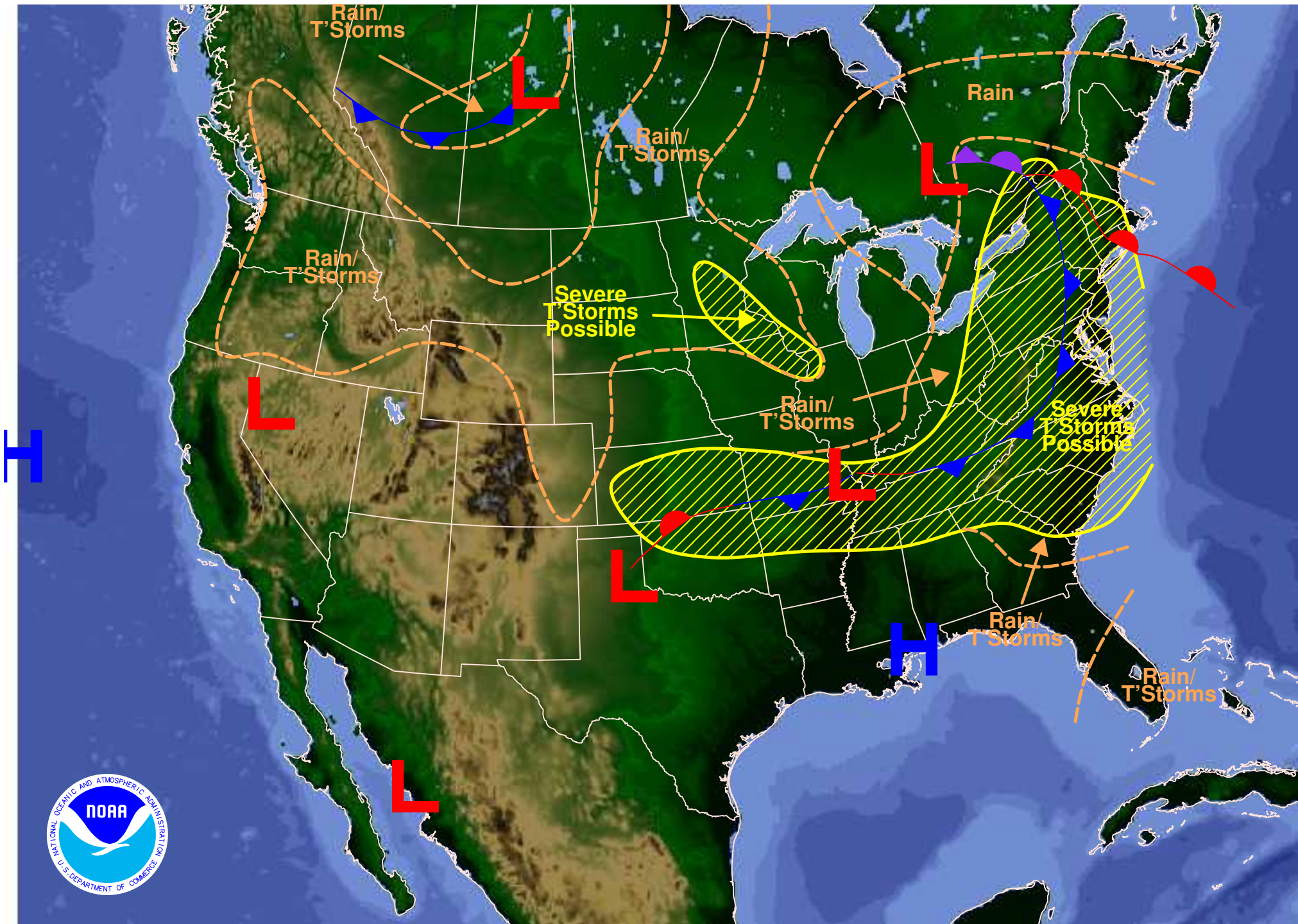
Weather Forecast for Saturday, May 31, 2008 DOC/NOAA/NWS/NCEP/Hydrometeorological Prediction Center Prepared by HEDGE based on HPC, SPC, and TPC forecasts.
