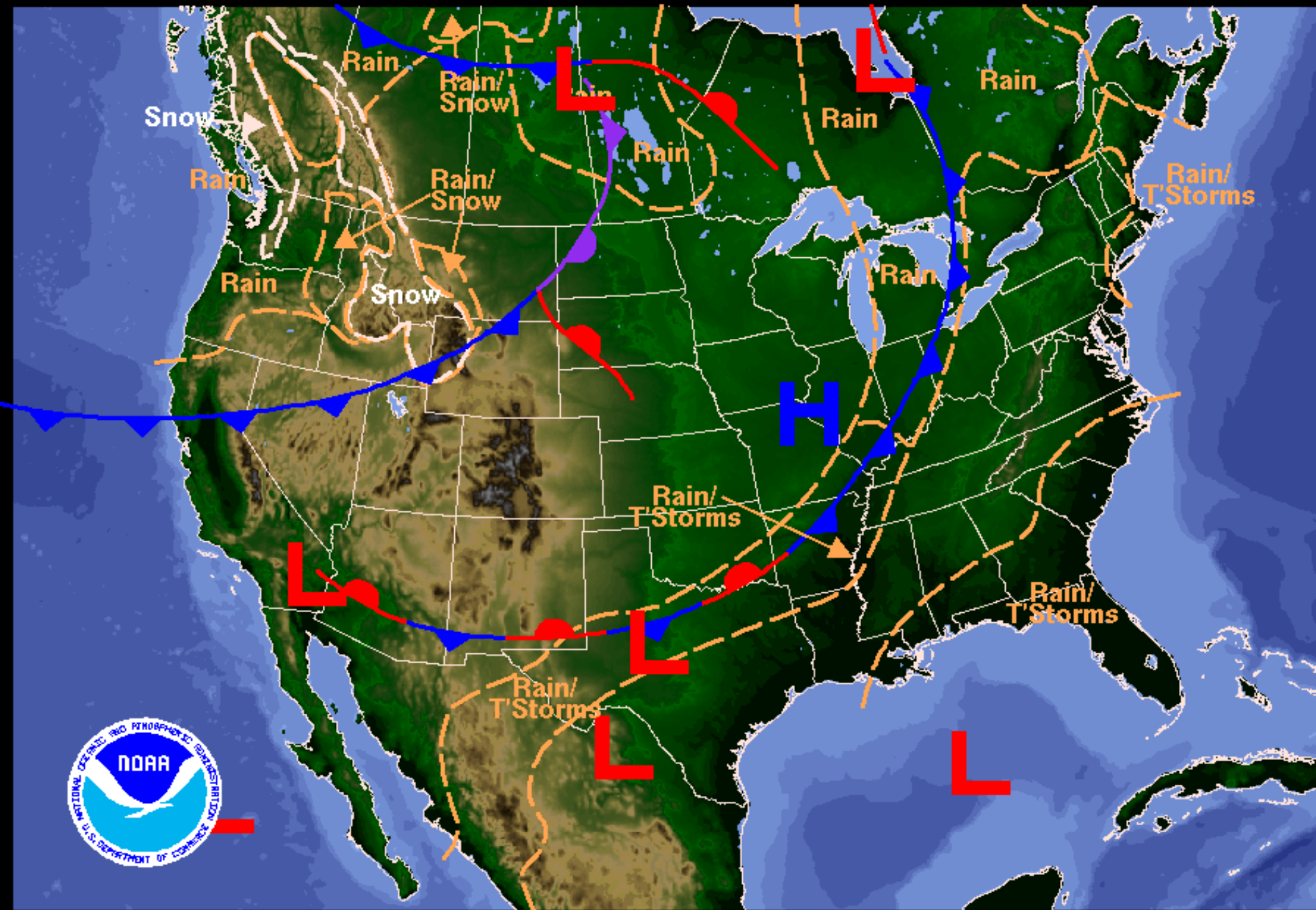
Weather Forecast for Wednesday, October 03, 2007 DOC/NOAA/NWS/NCEP/Hydrometeorological Prediction Center Prepared by Kocin based on HPC, SPC, and TPC forecasts.
