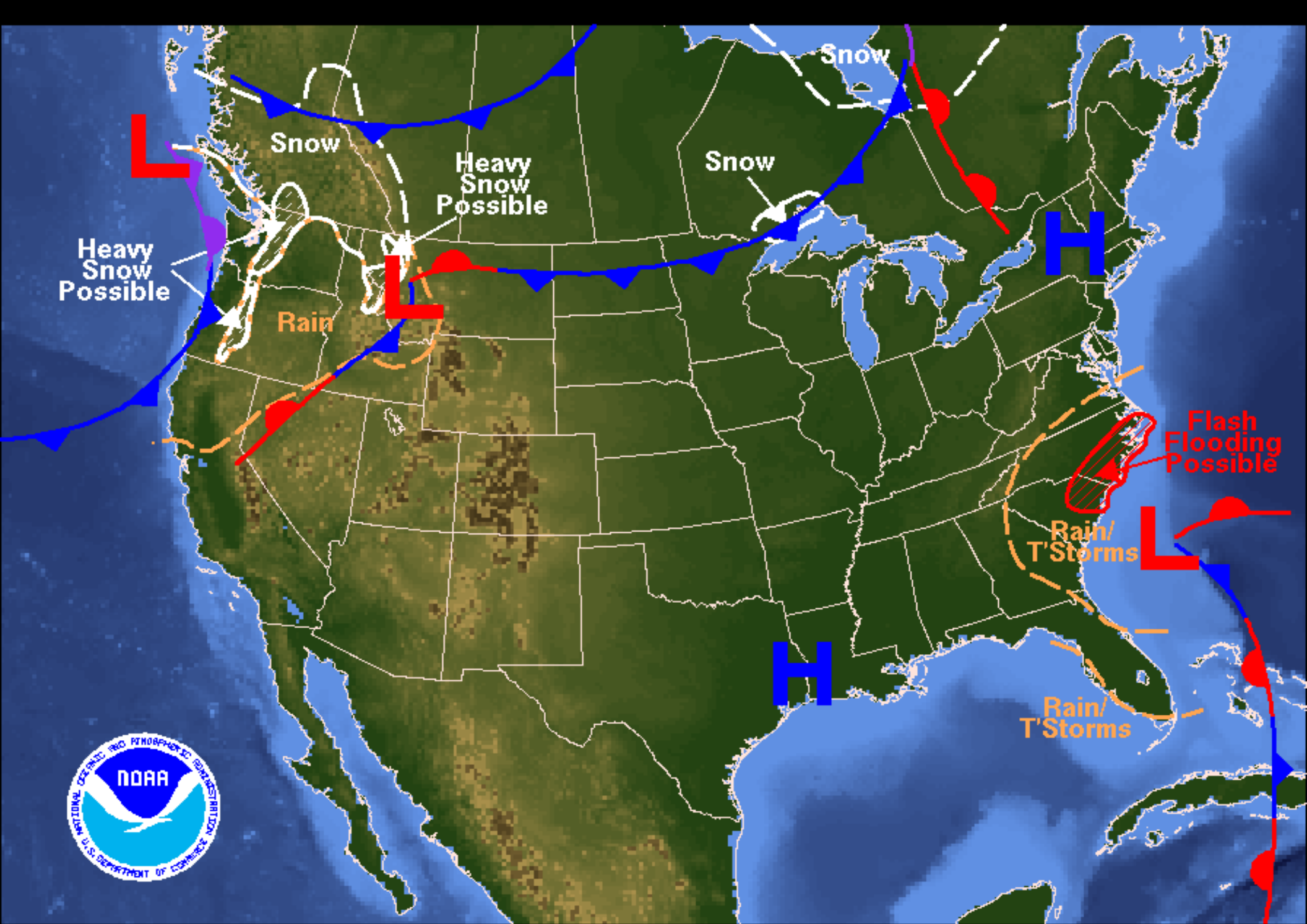
Weather Forecast for Tuesday, November 21, 2006 DOC/NOAA/NWS/NCEP/Hydrometeorological Prediction Center Prepared by Trimarco based on HPC, SPC, and TPC forecasts.
