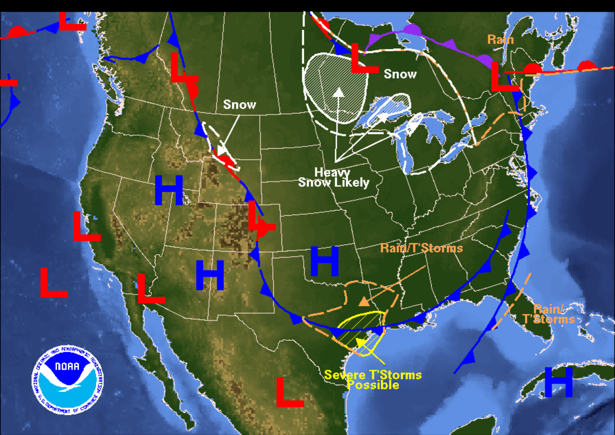
Weather Forecast for Thursday, October 12, 2006 DOC/NOAA/NWS/NCEP/Hydrometeorological Prediction Center Prepared by clark based on HPC, SPC, and TPC forecasts.
