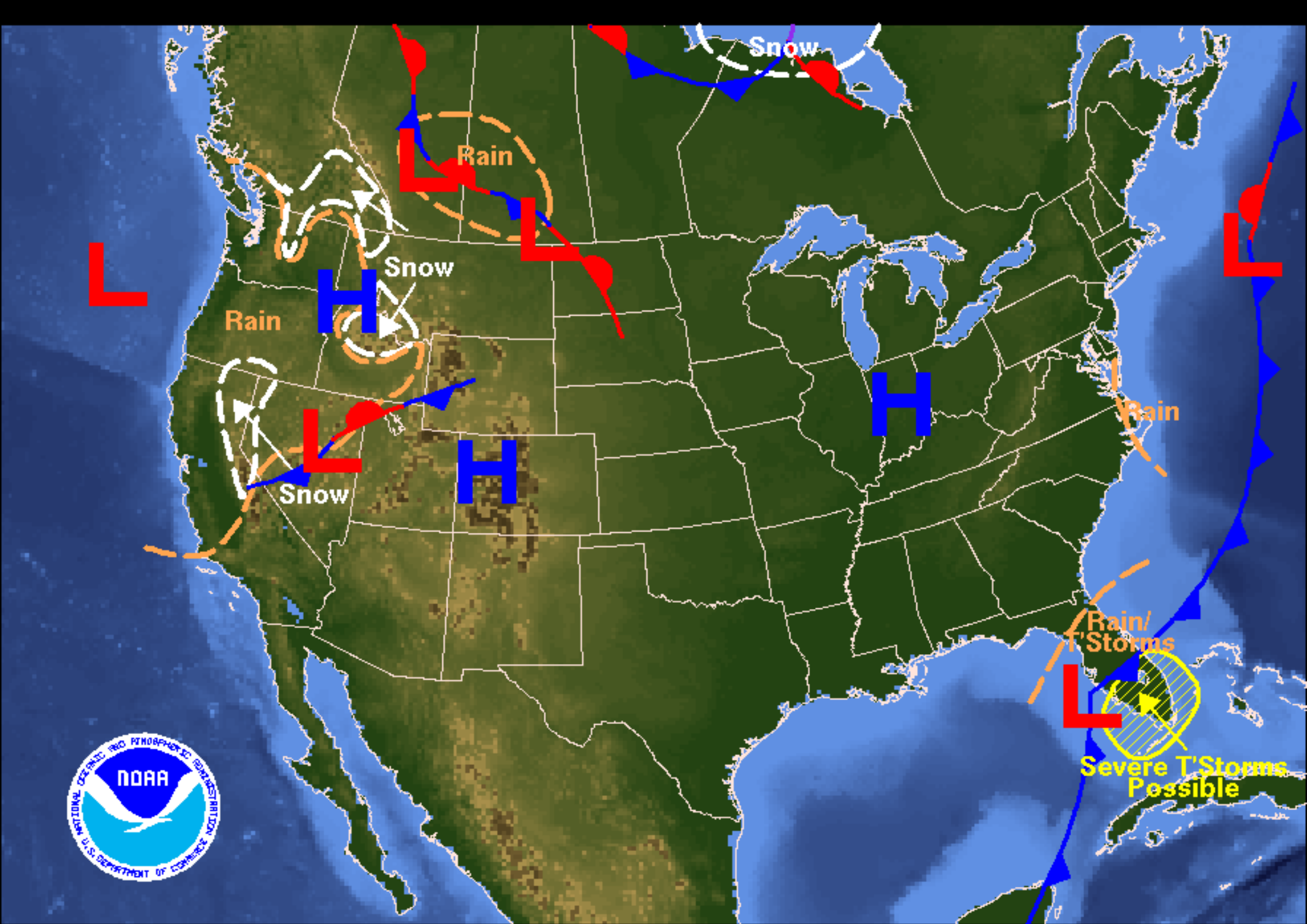
Weather Forecast for Sunday, April 09, 2006 DOC/NOAA/NWS/NCEP/Hydrometeorological Prediction Center Prepared by Lader based on HPC, SPC, and TPC forecasts.
