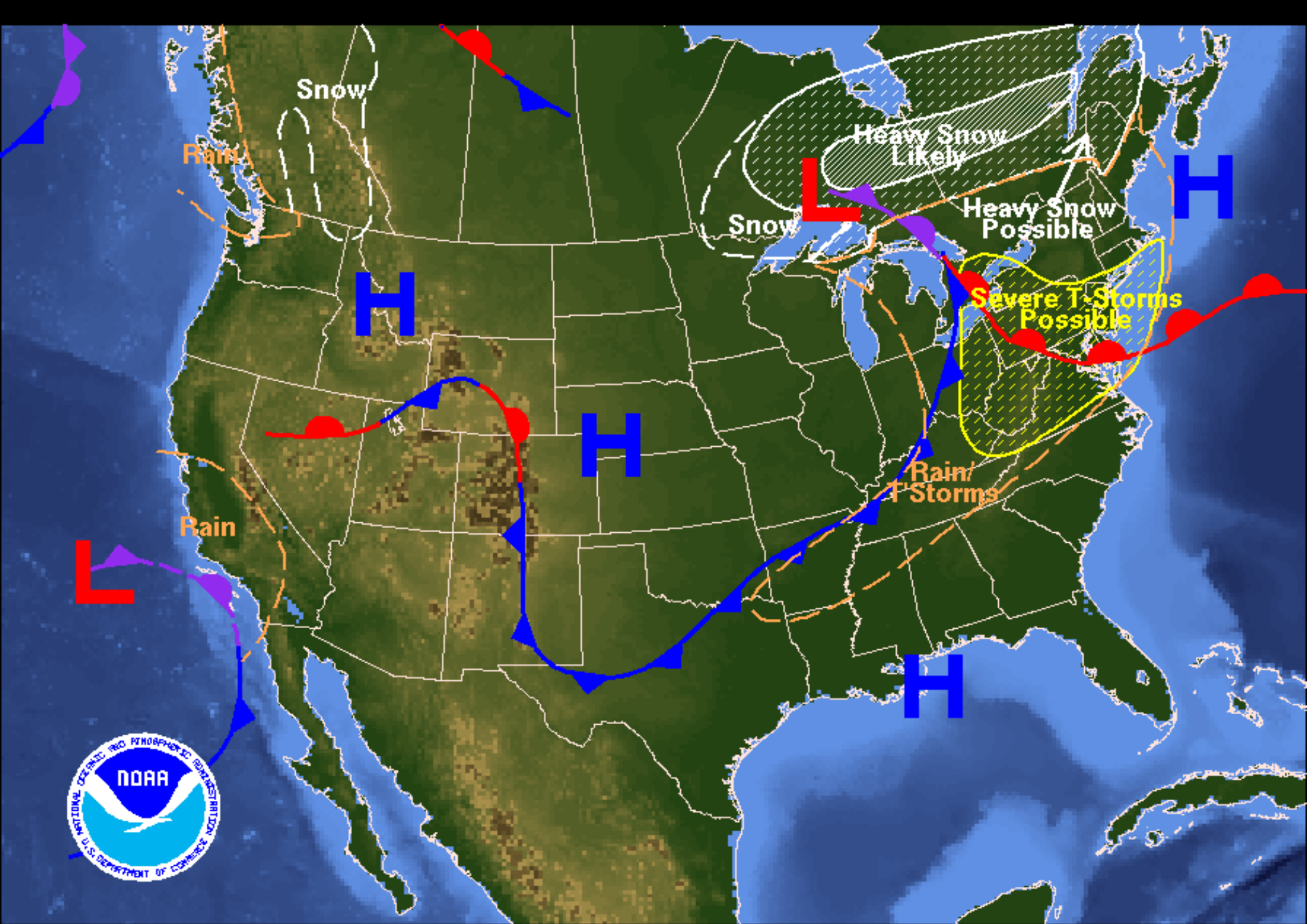
Weather Forecast for Wednesday, November 09, 2005 DOC/NOAA/NWS/NCEP/Hydrometeorological Prediction Center Prepared by Roth/Sullivan based on HPC, SPC, and TPC forecasts.
