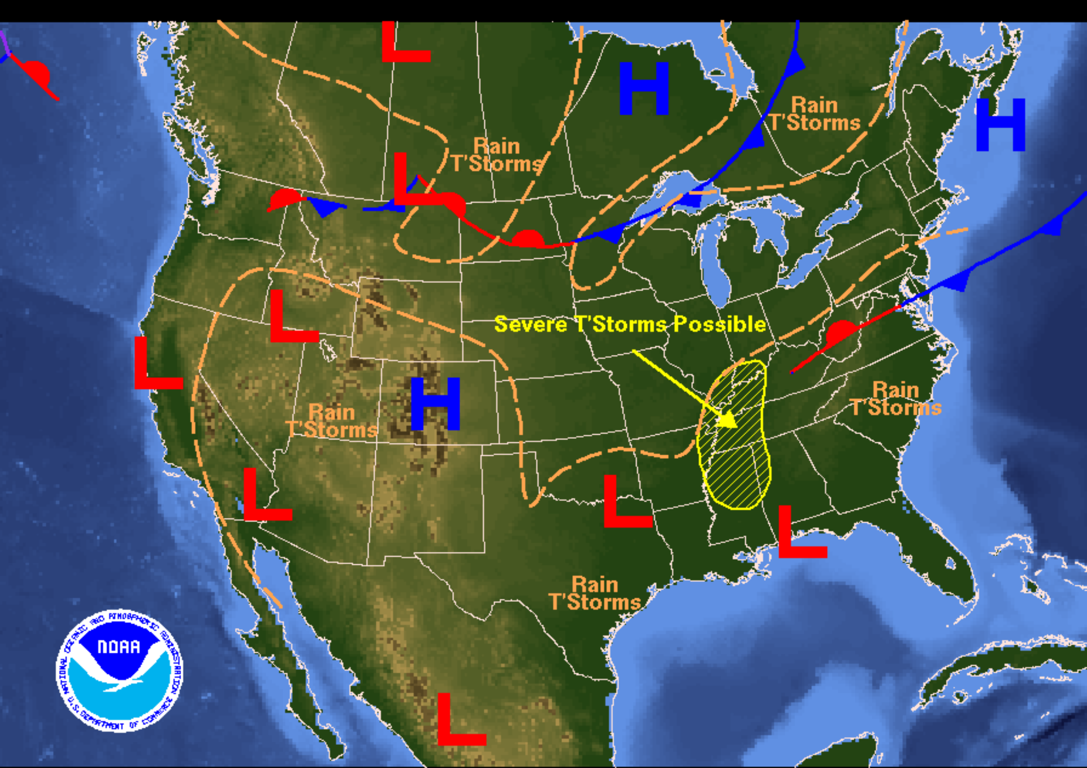
Weather Forecast for Sunday, August 07, 2005 DOC/NOAA/NWS/NCEP/Hydrometeorological Prediction Center Prepared by Clark/Oravec based on HPC, SPC, and TPC forecasts.
