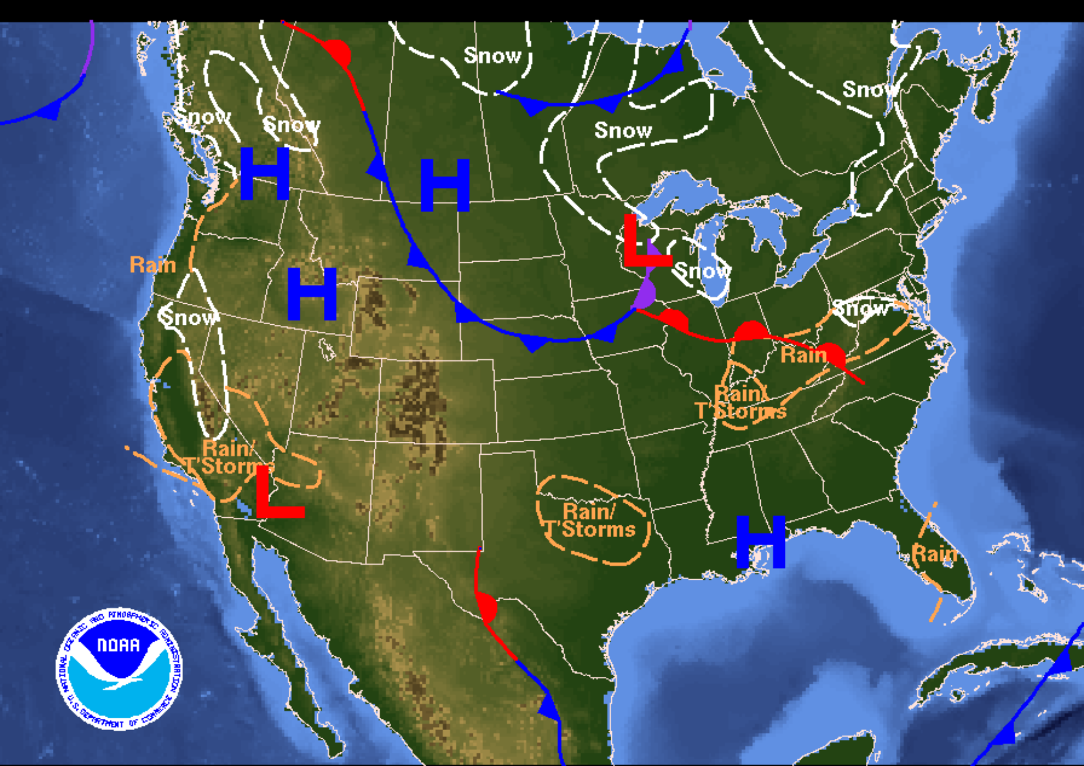
Weather Forecast for Friday, March 04, 2005 DOC/NOAA/NWS/NCEP/Hydrometeorological Prediction Center Prepared by Fries/Korty based on HPC, SPC, and TPC forecasts.
