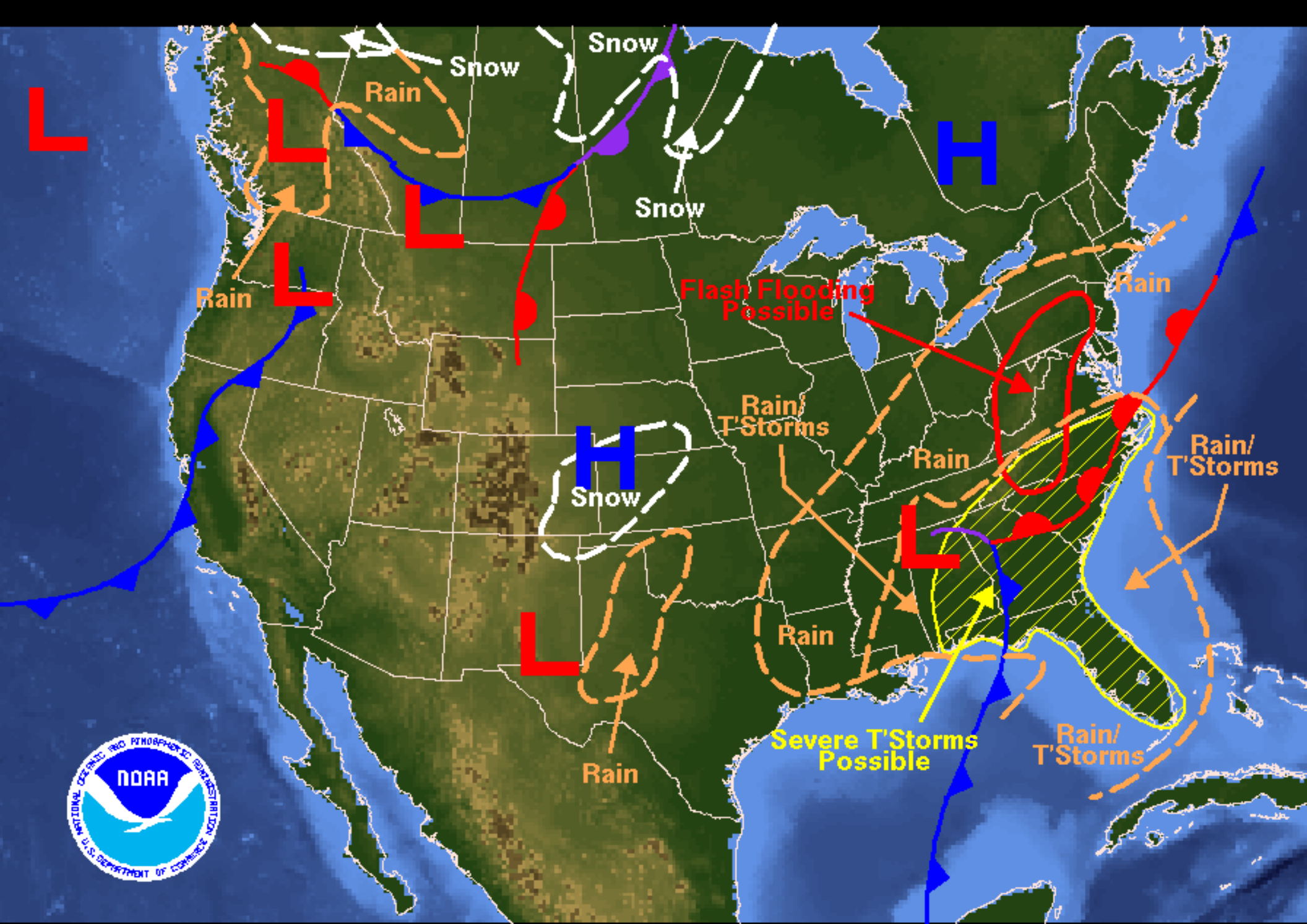
Weather Forecast for Monday, April 12, 2004 DOC/NOAA/NWS/NCEP/Hydrometeorological Prediction Center Prepared by Hatchett/Eckert based on HPC, SPC, and TPC forecasts.
