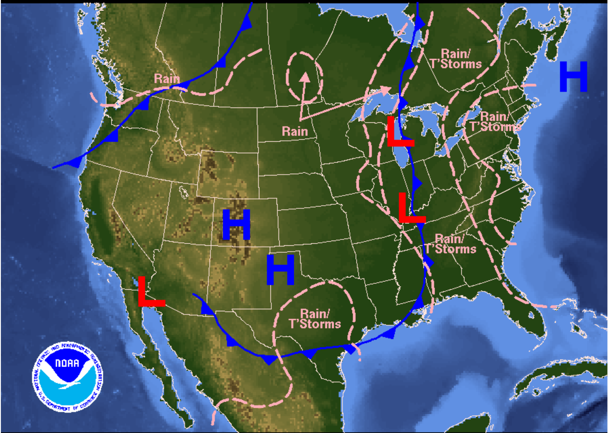
Weather Forecast for Sunday, September 14, 2003 DOC/NOAA/NWS/NCEP/Hydrometeorological Prediction Center Prepared by Hatchett/Eckert based on HPC, SPC, and TPC forecasts.
