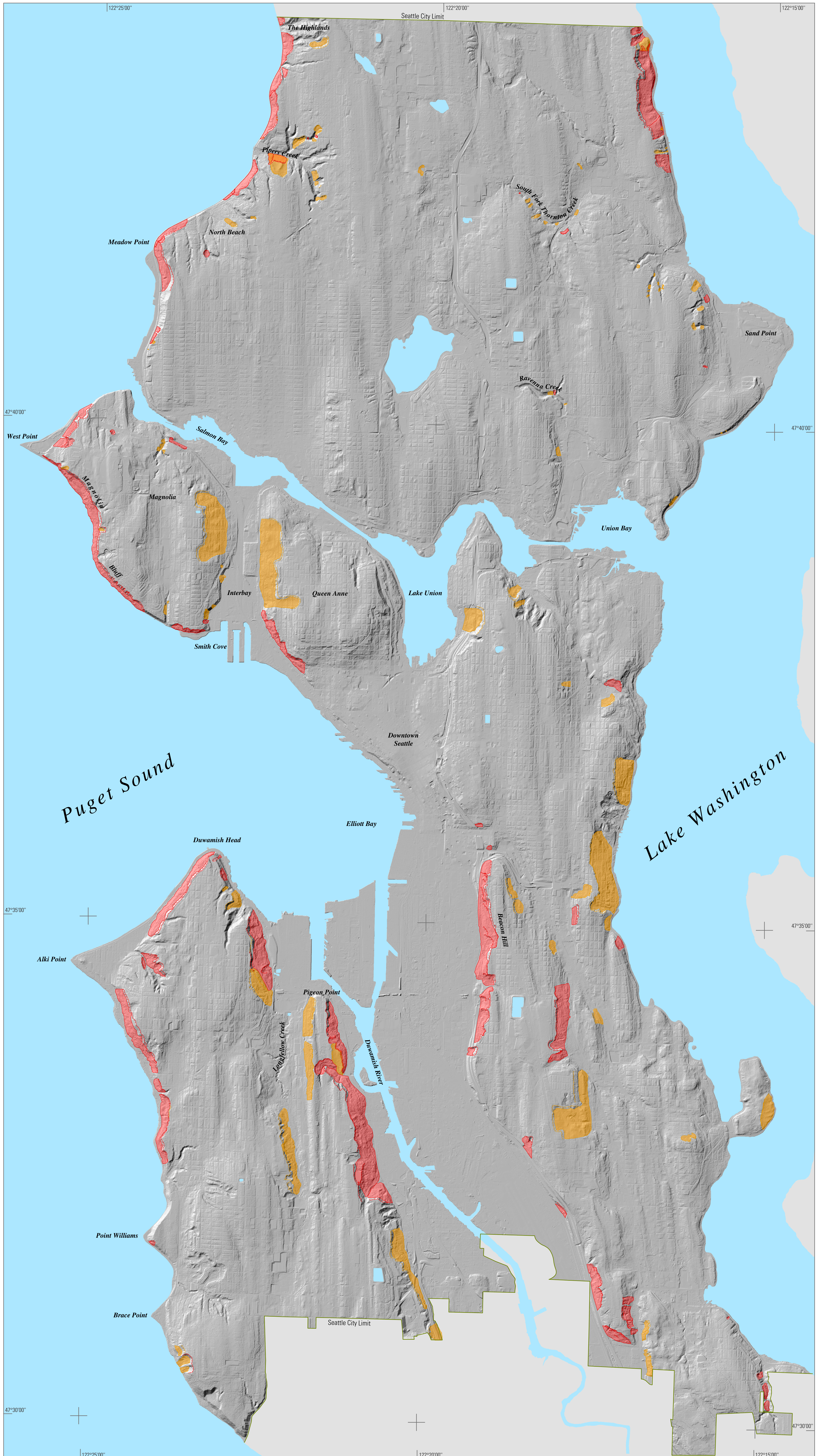
Base map is a shaded relief calculated from LIDAR-derived, 2-m digital elevation model. Virtual sun is 45° above the horizon and at an azimuth of 315°.
