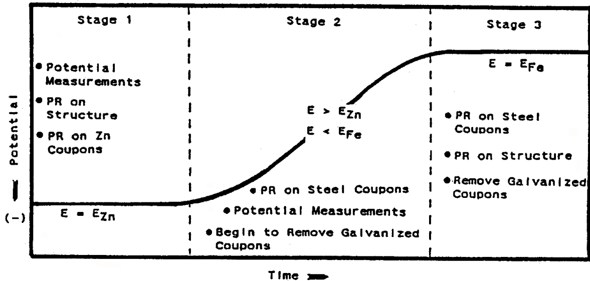
Figure 7. Stages of galvanized structure performance.
