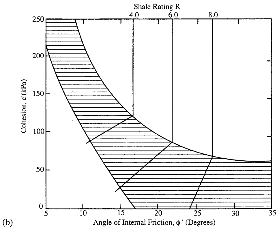
Figure 10-6: (a) Shale Rating System, (b) Trends in Shear-Strength Parameters of Compacted Shale Fills as a Function of Shale Quality. (Franklin, 1981)
