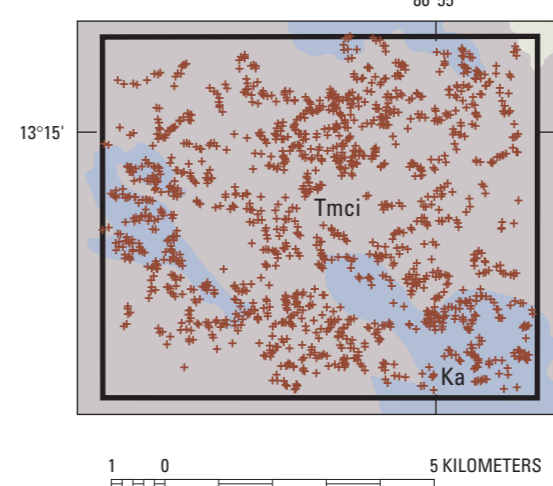
Map showing geologic units based on unpublished digital data provided by Instituto Nicaragüense de Estudios Territoriales (INETER) and the 1427 landslide initiation locations (crosses) within the study area.
