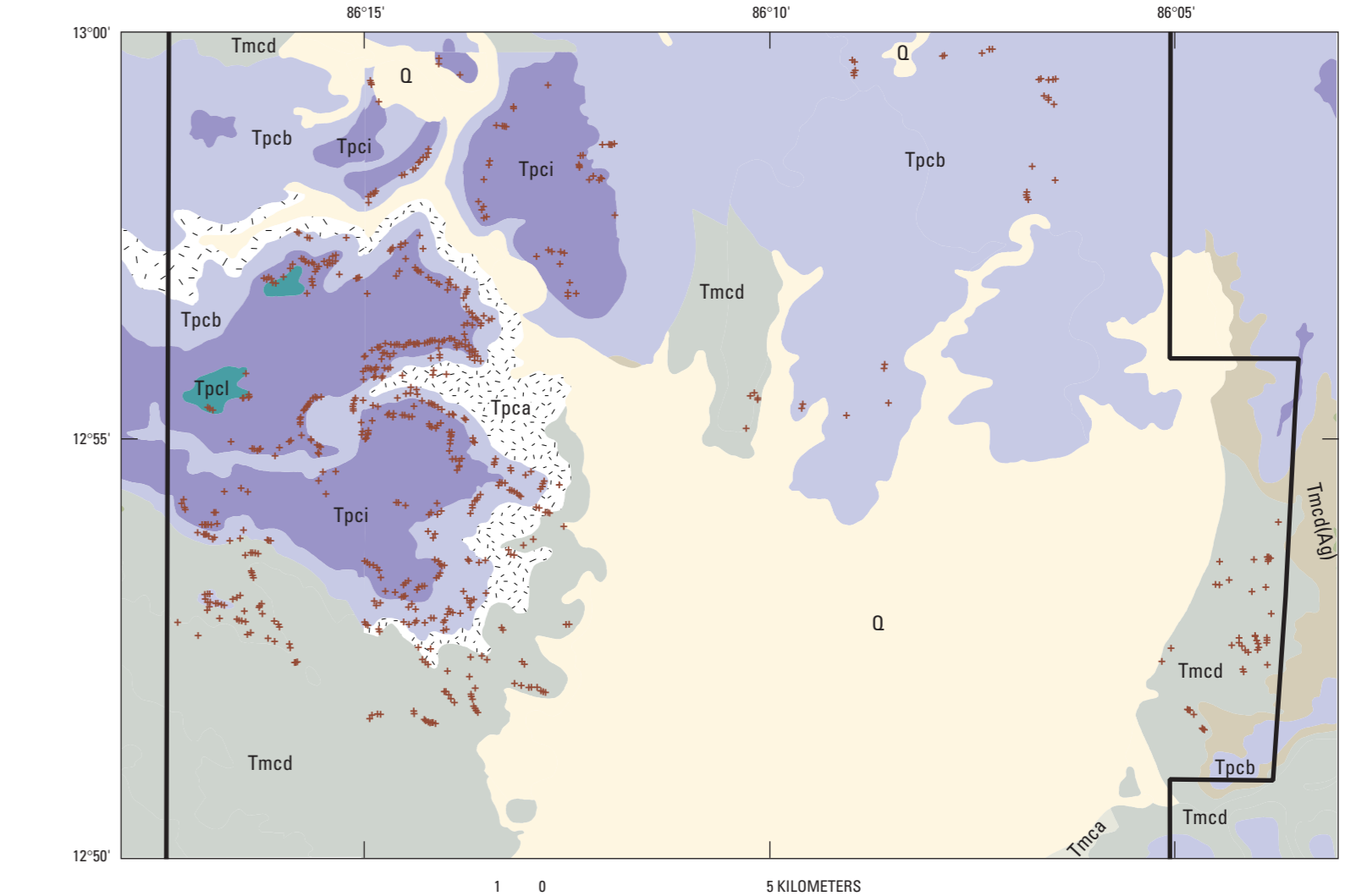
Map showing geologic units (R.L. Williams, G.H. Valery, and Carlos Birbuet, unpublished map) and the 655 landslide initiation locations (crosses) within the study area.
