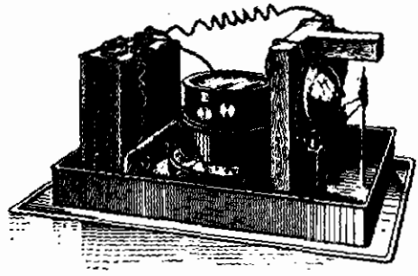
Popov's First Receiver - from Levizno -
