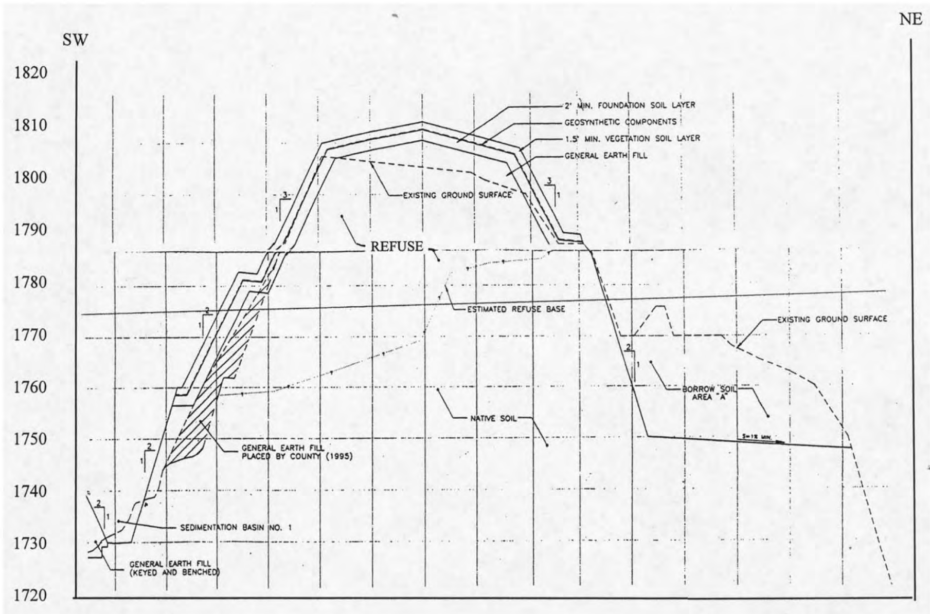
Figure 4. Laytonville Landfill Cross-Section Showing Height of Land, Refuse, and Cap, Laytonville, California
