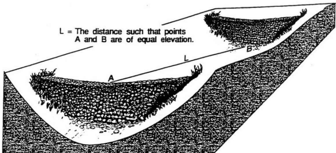
B. Spacing between rock check dams.
