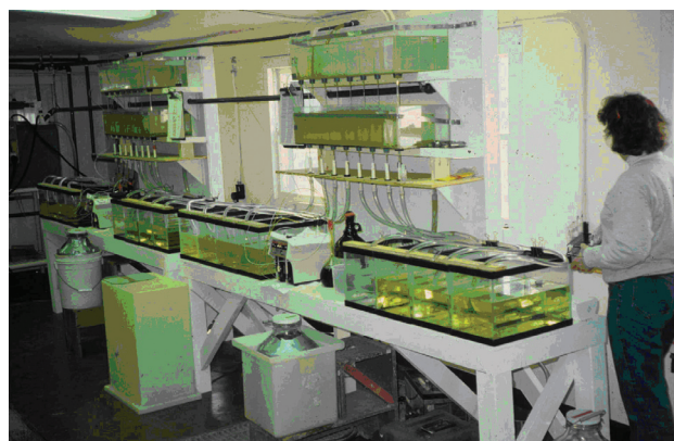
Figure 3. Photograph of the continuous-flow dilution system used to assess the toxicity of the lampricides on the three mussel species in relation to larval sea lampreys ( Petromyzon marinus ).
