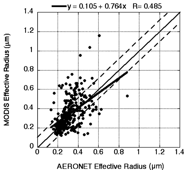
FIG. 12. MODIS-retrieved aerosol particle effective radius over ocean plotted against AERONET retrievals of the same parameter. Only points with AERONET \tau_{0.44} > 0.15 are plotted. AERONET values are daily averages for the date of the MODIS overpass. The blue line represents the linear regression through the points, the solid black line is the 1:1 line, and the dashed lines represent \pm 0.10 \mu\text{m} ; 271 collocated points are shown, and 62% of these points fall within the dashed lines.
