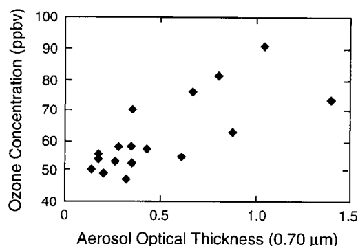
Figure 11. Average ozone concentration (from 1000 to 500 mbar) as function of the aerosol optical thickness, AOT (0.70 \mu\text{m} channel). A split pattern is observed due to a change in the air circulation pattern.
