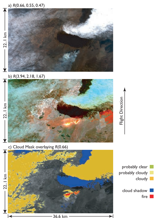
Figure 6. These MAS images of a prescribed fire and nearby clouds were acquired over the Madikwe Private Game Reserve, South Africa, on 20 August 2000. (a) True color RGB composite of bands at 0.66, 0.55, and 0.47 \mu\text{m} . (b) False color composite of bands at 3.94, 2.18, and 1.67 \mu\text{m} . (c) Resultant cloud, shadow, and fire mask. All images have been resampled to a constant spatial resolution of 64 m resolution. The thermal emission of the hot fire line clearly shows up beneath the smoke using the shortwave infrared bands.
