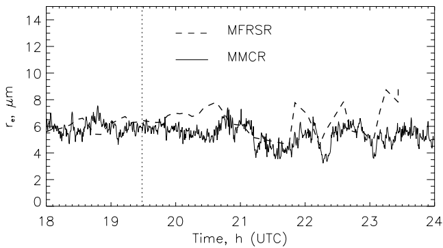
Figure 5. Time series of r_e derived from the surface-based MFRSR and MMCR at SGP. The time of the Twin Otter aircraft overflight is marked by a vertical dotted line.
