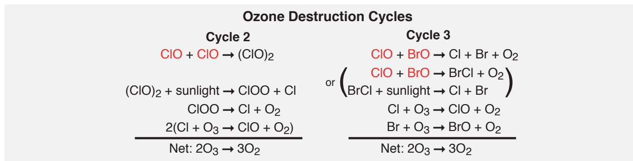
Figure Q9-2. Polar ozone destruction Cycles 2 and 3. Significant destruction of ozone occurs in polar regions because ClO abundances reach large values. In that case, the cycles initiated by the reaction of ClO with another ClO (Cycle 2) or the reaction of ClO with BrO (Cycle 3) efficiently destroy ozone. The net reaction in both cases is two ozone molecules forming three oxygen molecules. The reaction of ClO with BrO has two pathways to form the Cl and Br product gases. Ozone destruction Cycles 2 and 3 are catalytic, as illustrated for Cycle 1 in Figure Q9-1 , because chlorine and bromine react and are reformed in each cycle. Sunlight is required to complete each cycle and to help form and maintain ClO abundances.
