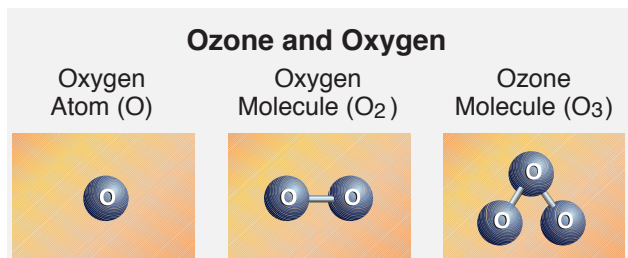
Figure Q1-1. Ozone and oxygen. A molecule of ozone (O 3 ) contains three oxygen (O) atoms bound together. Oxygen molecules (O 2 ), which constitute 21% of Earth’s atmosphere, contain two oxygen atoms bound together.
