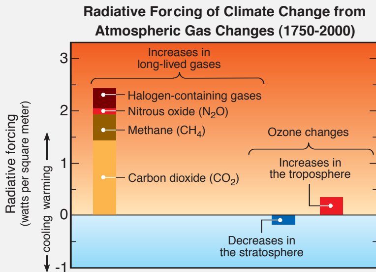
Figure Q18-1. Climate change from atmospheric gas changes. Human activities since 1750 have caused increases in the abundances of several long-lived gases, changing the radiative balance of Earth’s atmosphere. These gases, known as “greenhouse gases,” result in radiative forcings , which can lead to climate change. The largest radiative forcings come from carbon dioxide, followed by methane, tropospheric ozone, the halogen-containing gases (see Figure Q7-1 ), and nitrous oxide. Ozone increases in the troposphere result from pollution associated with human activities. All these forcings are positive, which leads to a warming of Earth’s surface. In contrast, stratospheric ozone depletion represents a small negative forcing, which leads to cooling of Earth’s surface. In the coming decades, halogen gas abundances and stratospheric ozone depletion are expected to be reduced along with their associated radiative forcings. The link between these two forcing terms is an important aspect of the radiative forcing of climate change.
