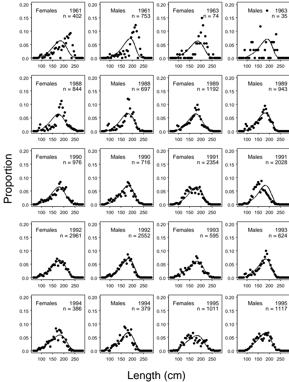
Figure 13.2. Observed (points) and fitted (lines) catch-at-length proportions by sex in the NF-Gulf region up to 1998. Line symbolism is the same as Figure 9. All fits are virtually identical.
