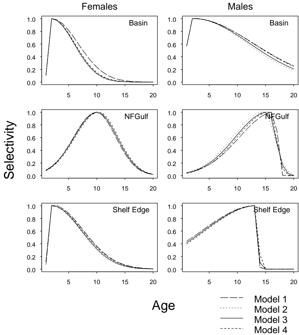
Figure 9. Estimated selectivity curves for porbeagle fisheries in three regions obtained from the four models (see text).
