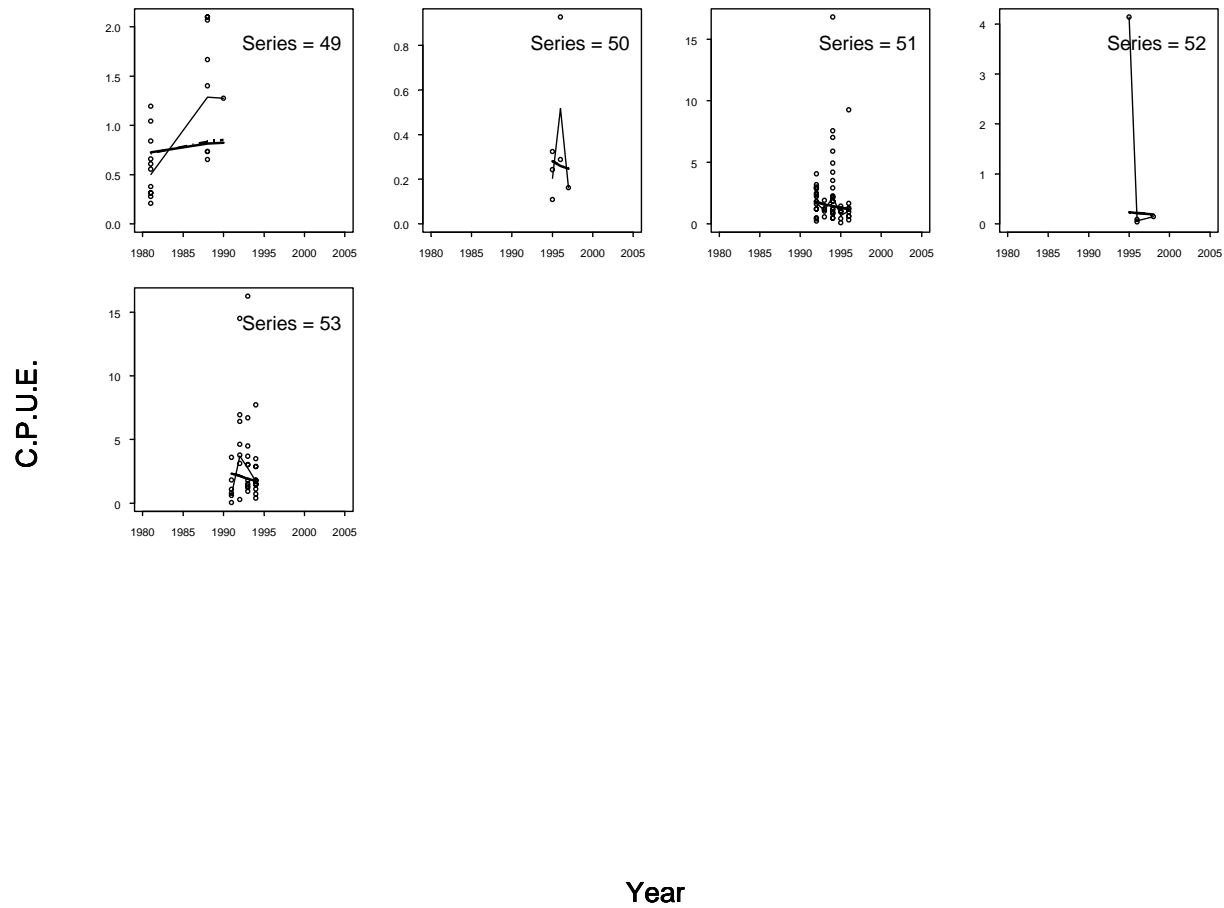
Figure 11.5. Observed (points) and fitted (lines) catch per unit effort by weight for each porbeagle CPUE series (a single vessel fishing in a single area during a single season). The light line is the annual geometric mean of the data. The dark line is the model fit obtained from Model 3.
