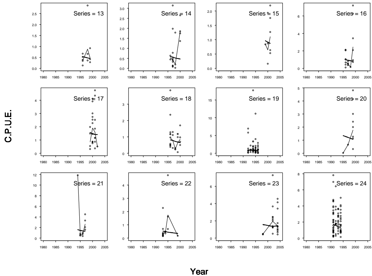
Figure 11.2. Observed (points) and fitted (lines) catch per unit effort by weight for each porbeagle CPUE series (a single vessel fishing in a single area during a single season). The light line is the annual geometric mean of the data. The dark line is the model fit obtained from Model 3.
