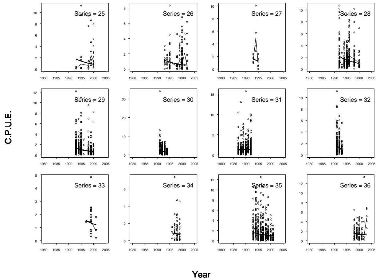
Figure 11.3. Observed (points) and fitted (lines) catch per unit effort by weight for each porbeagle CPUE series (a single vessel fishing in a single area during a single season). The light line is the annual geometric mean of the data. The dark line is the model fit obtained from Model 3.
