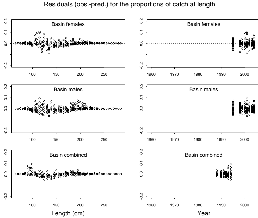
Figure 14.1. Raw residuals for fits to the catch-at-length data by length and by year for the Basin region obtained from Model 3.
