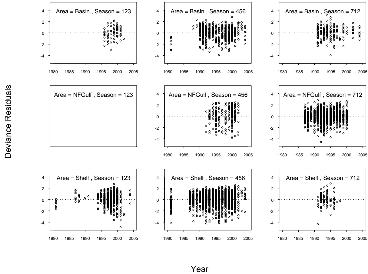
Figure 12. Deviance residuals for the fits to the CPUE data by season and area, obtained from Model 3.
