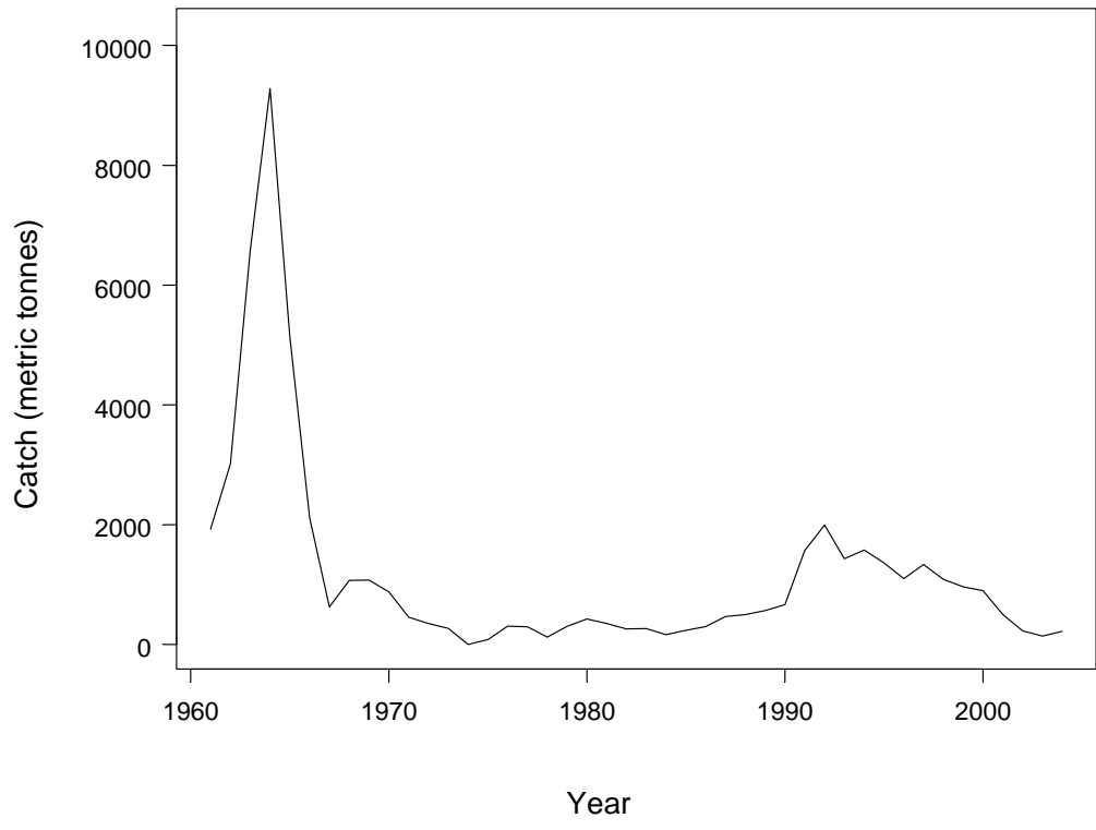
Figure 1. Porbeagle landings in northwest Atlantic (NAFO Areas 2-6) from 1961 to 2005.
