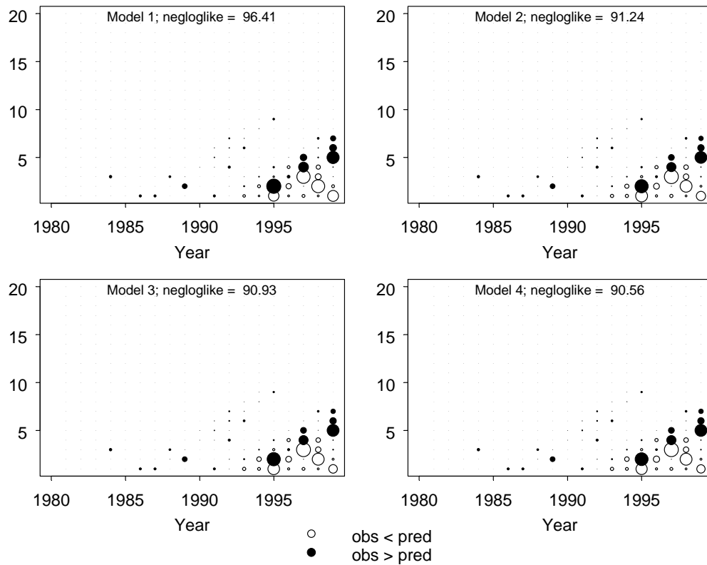
Figure 16. Residuals (observed tag recaptures - predicted tag recaptures) for the tagging component of the model. Points are proportional in size to the size of the residual (max. 12.5).
