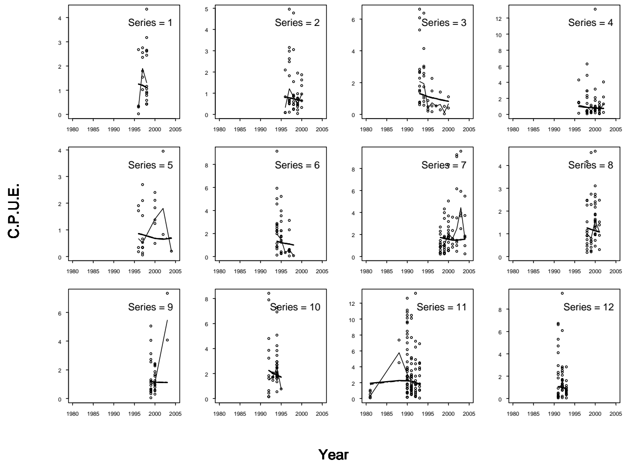
Figure 11.1. Observed (points) and fitted (lines) catch per unit effort by weight for each porbeagle CPUE series (a single vessel fishing in a single area during a single season). The light line is the annual geometric mean of the data. The dark line is the model fit obtained from Model 3.
