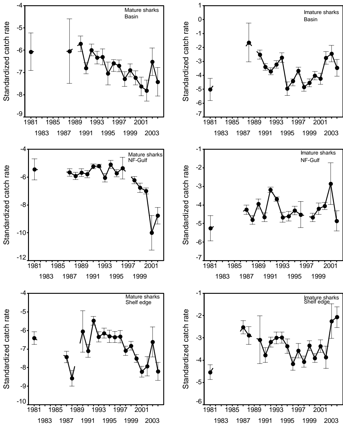
Figure 8. Standardized catch rate (log C.P.U.E) for mature and immature porbeagle in the 3 regions. Error bars are 95% confidence intervals.
