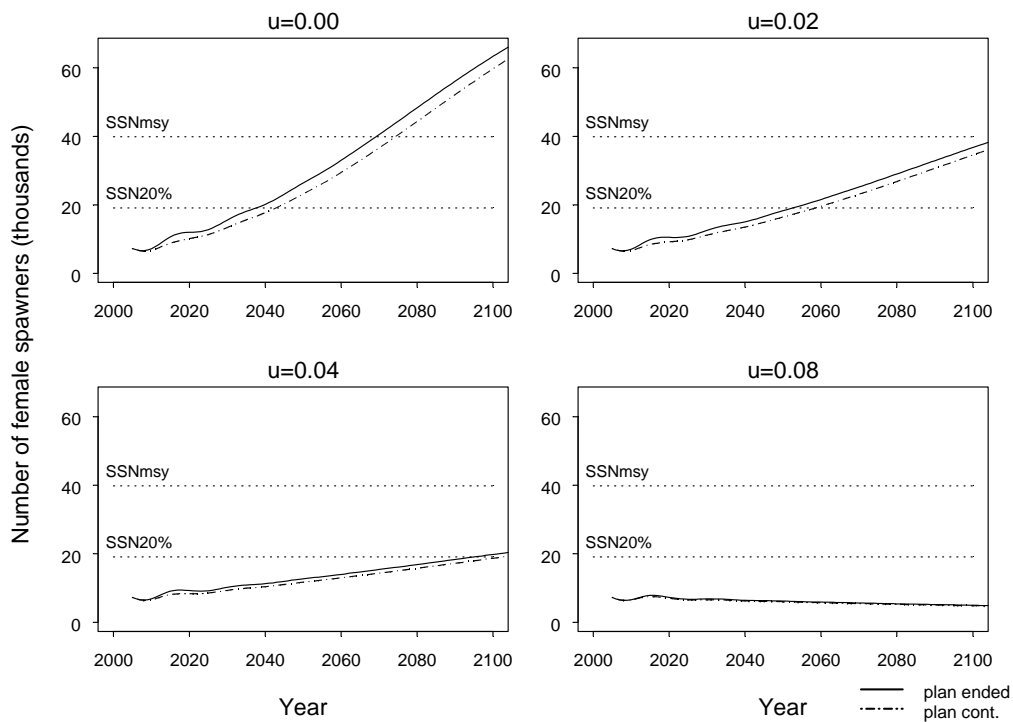
Figure 22. Comparison of the predicted recovery trajectories under two management scenarios based on Model 1. The solid line indicates the recovery trajectories if the current management 5 year plan ended at the end of 2005 (3 years into the plan) and porbeagle were managed under SARA after that time. “ u ” is the exploitation rate corresponded to different levels of human-induced mortality. The dashed line indicates the recovery trajectory if the current management plan was allowed to continue for the duration of the plan (ending at the end of 2007), and management of the population was under SARA after that time. Population projections begin in 2005 from the abundance by age and sex predicted by the model, and are projected deterministically using the life history parameters obtained from the model and the assumed exploitation rate. The Shelf-Edge selectivity is used for the projections.
