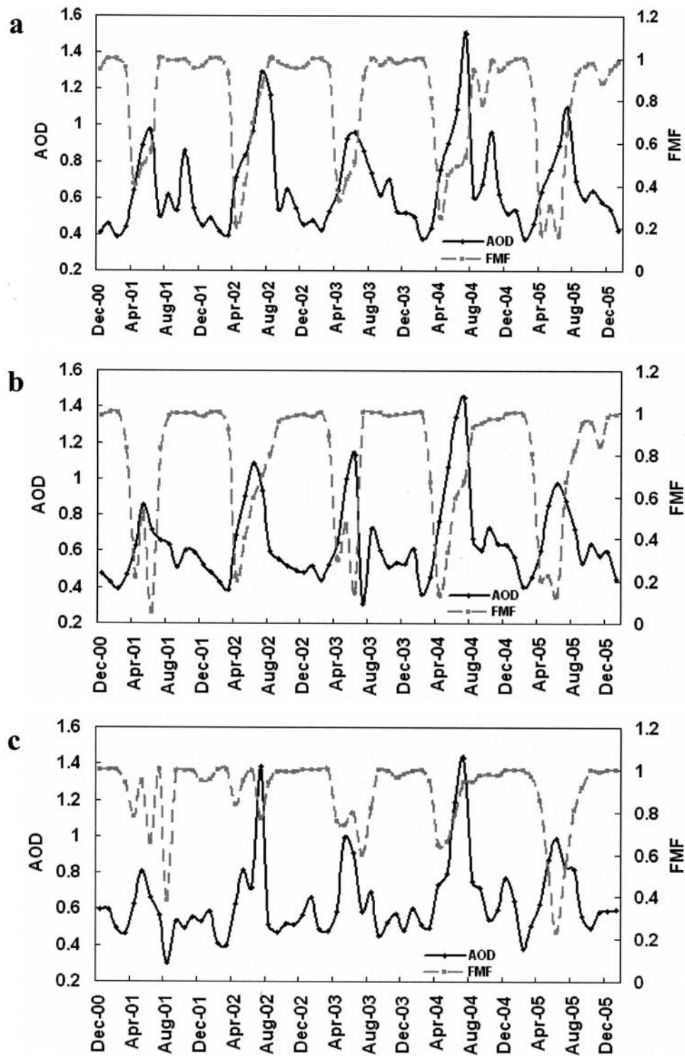
Figure 2. Variations of AOD and FMF over three cities in the IG plains: (a) New Delhi, (b) Kanpur, and (c) Patna.
