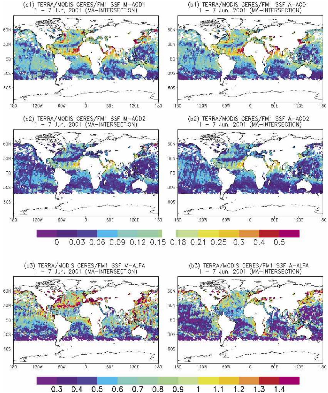
FIG. 8. Distribution in MA intersection of [a(1), b(1)] \tau_1 , [a(2), b(2)] \tau_2 , and [a(3), b(3)] \alpha derived from Terra CERES/FM1 SSF in Jun 2001: (left) M product and (right) A product. Compare with distributions in the MA intersection in Dec 2000: \tau_1 in Figs. 2a(2)–b(2); \tau_2 in Figs. 3a(2)–b(2); and \alpha in Figs. 4a(2)–b(2). (See discussion in section 3e.)
