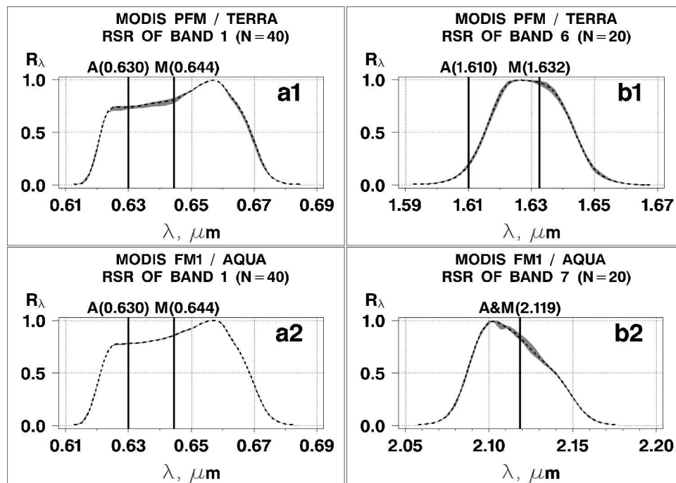
FIG. A1. RSR of the MODIS bands used in the AVHRR-like retrievals (a) 1 and (b) 6(7) on (top) Terra and (bottom) Aqua . Superimposed are reference wavelengths at which the A and M products are reported. (Solid lines represent average RSRs over the 40/20 detectors, and shaded areas show cross-detector variability.)
