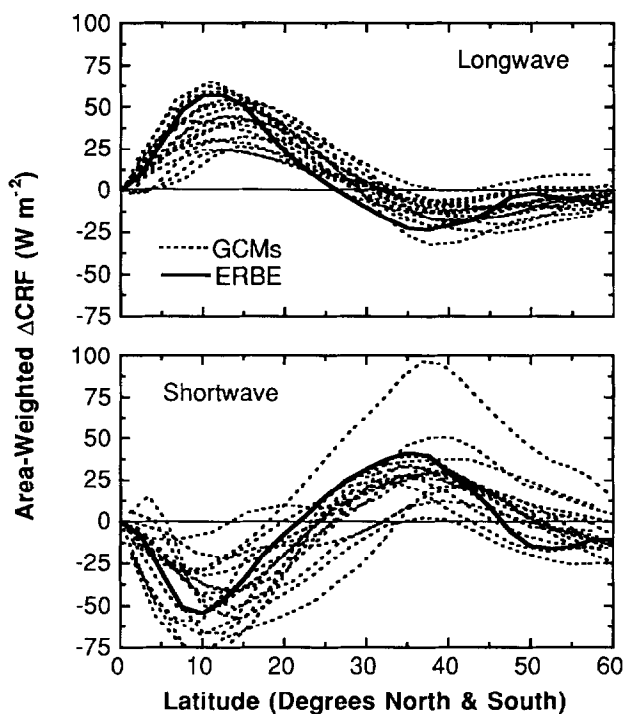
FIG. 4. Comparison of zonal-mean DCRF for 17 GCMs to the ERBE data. These represent 4-yr means.
