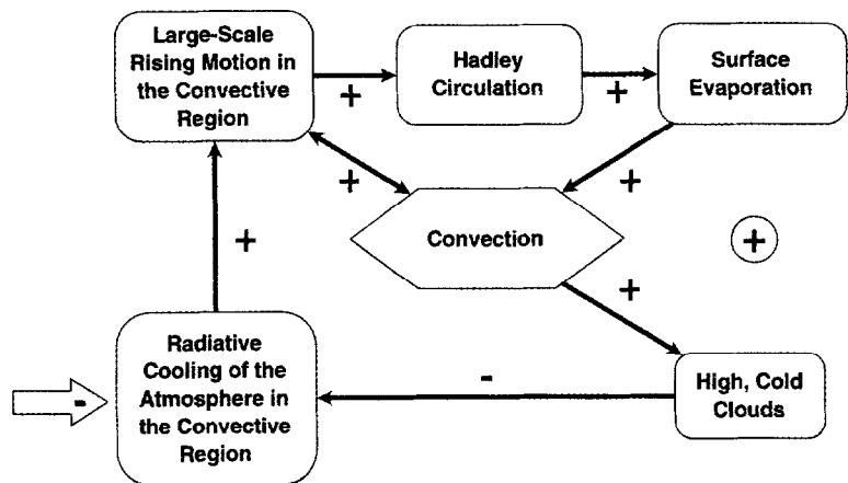
FIG. 7. Schematic diagram illustrating the RDC feedback loop.
