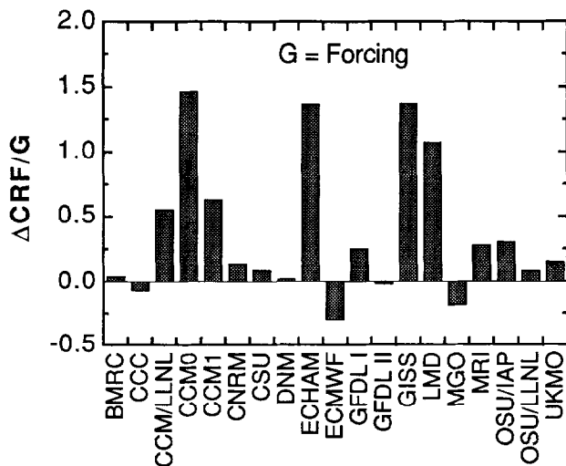
FIG. 3. The cloud feedback parameter \Delta\text{CRF}/G , as produced by 19 atmospheric GCMs (Cess et al. 1990).
