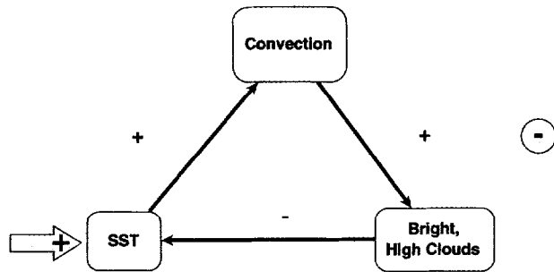
FIG. 6. Schematic figure illustrating the thermostat effect hypothesized by Ramanathan and Collins (1991).
