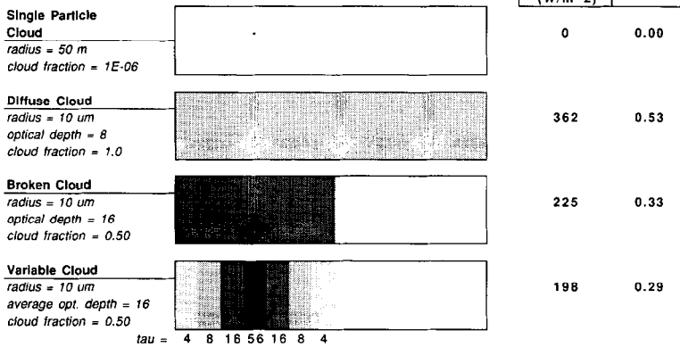
FIG. 9. Schematic diagram of varying distributions of cloud liquid water in a global climate model, and their impact on calculations of TOA SW reflected fluxes. All cases have equal total liquid water.
