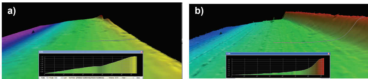
Fig. 2: Sample data from slope area. Shown are a) MBES data and b) PDBS data (GeoAcoustics GeoSwath). Note that while the PDBS data is noisier than the MBES it still captures the small feature in the upper left portion of the data and the small depressions along the base of the slope. The along track artifacts are on the order of 0.1m in amplitude. Data is shown with a vertical exaggeration of 6.
