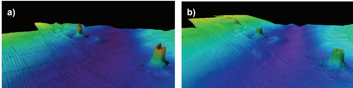
Fig. 3: Shown are bridge abutments as modeled from a) MBES and b) PDBS (GeoAcoustics GeoSwath) data. Note the submerged cable trenches running parallel to the bridge and the remnant of a cofferdam at the base of the abutment in the lower right corner of each image. The motion artifacts clearly visible in the MBES data were the result of pole motion. Data are shown without vertical exaggeration.
