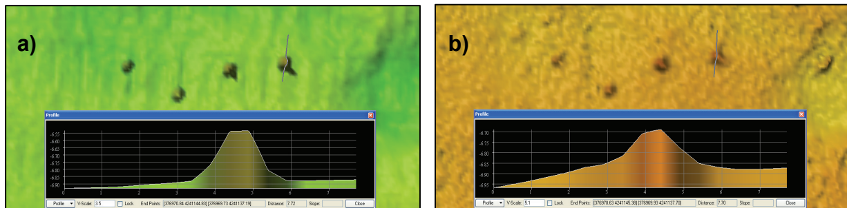
Fig. 1: Sonar targets as gridded from a) MBES data and b) PDBS (GeoAcoustics GeoSwath) data. Note that the gridding process has reduced the height of the target in both datasets and that while the effect is more dramatic in the PDBS data the targets remain readily visible. Data are shown with a vertical exaggeration of 6.
