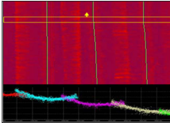
Figure 4.10: HIPS Subset Editor view (bottom) of acoustic refraction-induced bathymetry errors, using BASE surface standard deviation image for reference.
