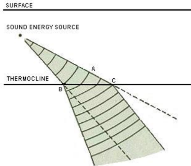
Figure 4.8: Sonar refraction due to thermocline.
