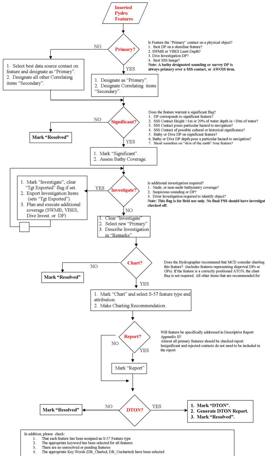
Figure 4.24: Pydro data flagging decision tree.
