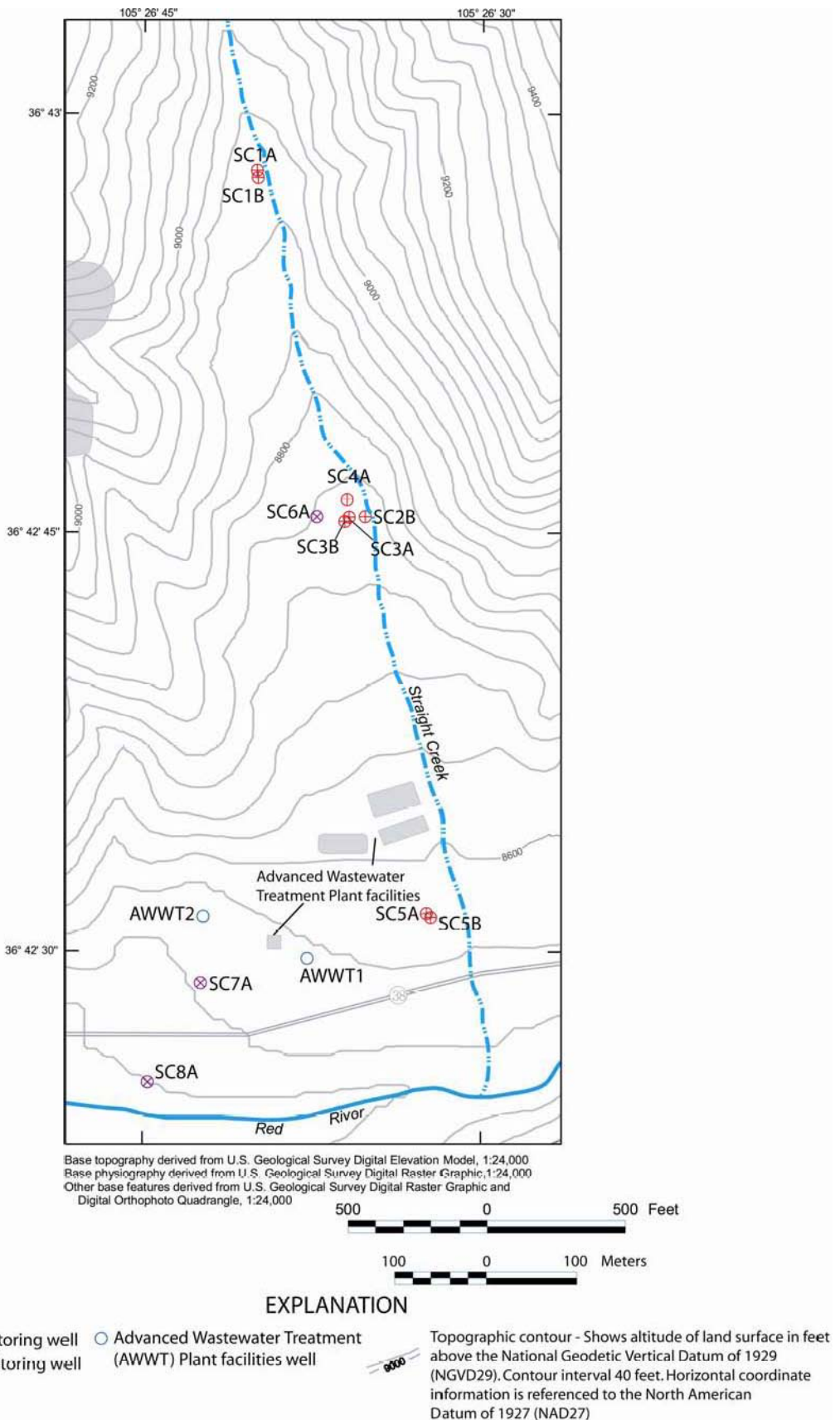
Figure 2. Map showing locations of monitoring wells in the Straight Creek catchment.
