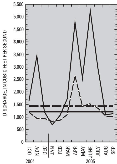
05079000 RED LAKE RIVER AT CROOKSTON DRAINAGE AREA 5,270 SQUARE MILES
