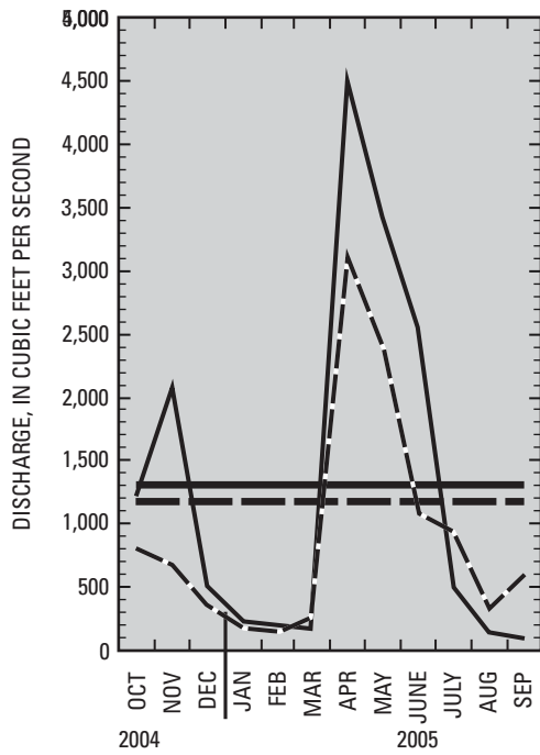
05131500 LITTLE FORK RIVER AT LITTLEFORK DRAINAGE AREA 1,680 SQUARE MILES
