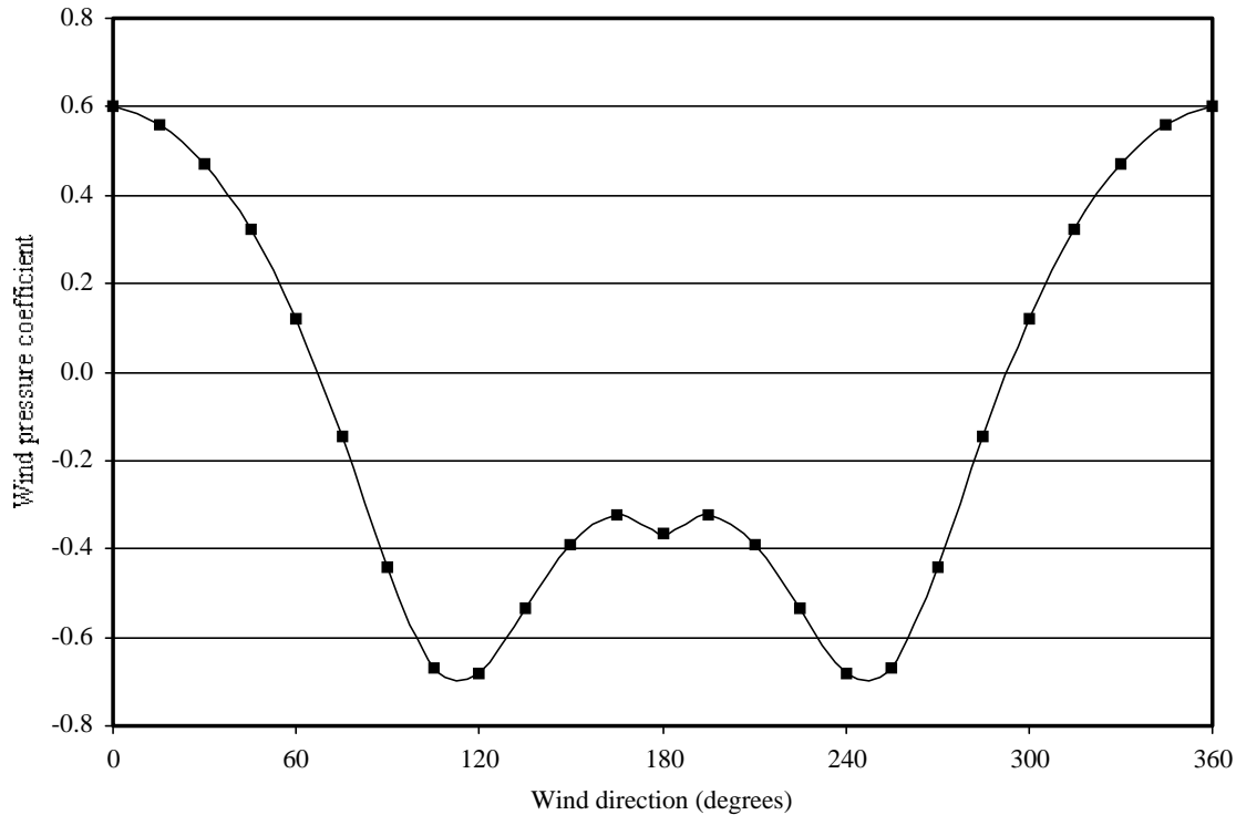
Figure 1 Plot of Wind Pressure Profile in Table 3
