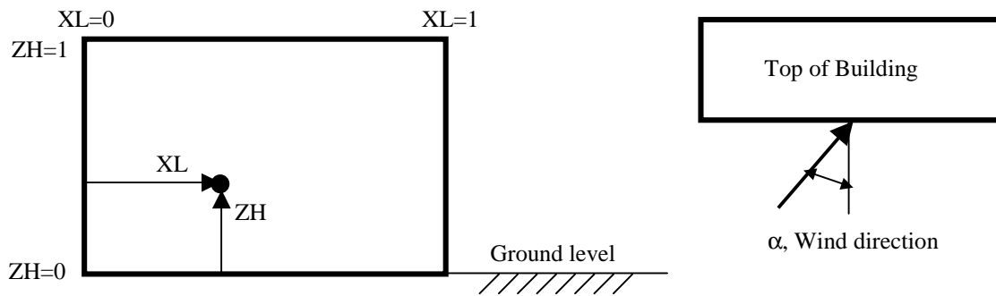
Figure 2 Determination of Tall Building Wind Pressure Coefficients
