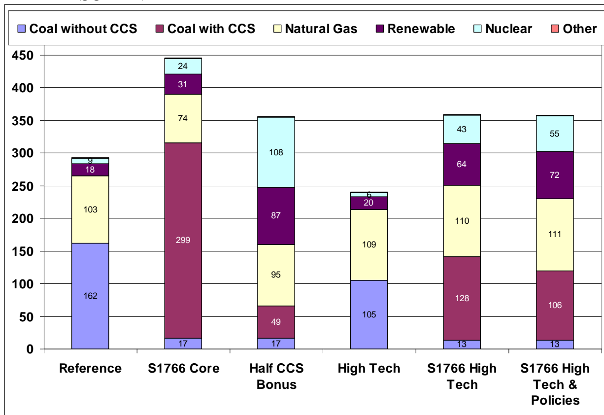
Figure 11: Cumulative Electricity Generating Capacity Additions (gigawatts)
