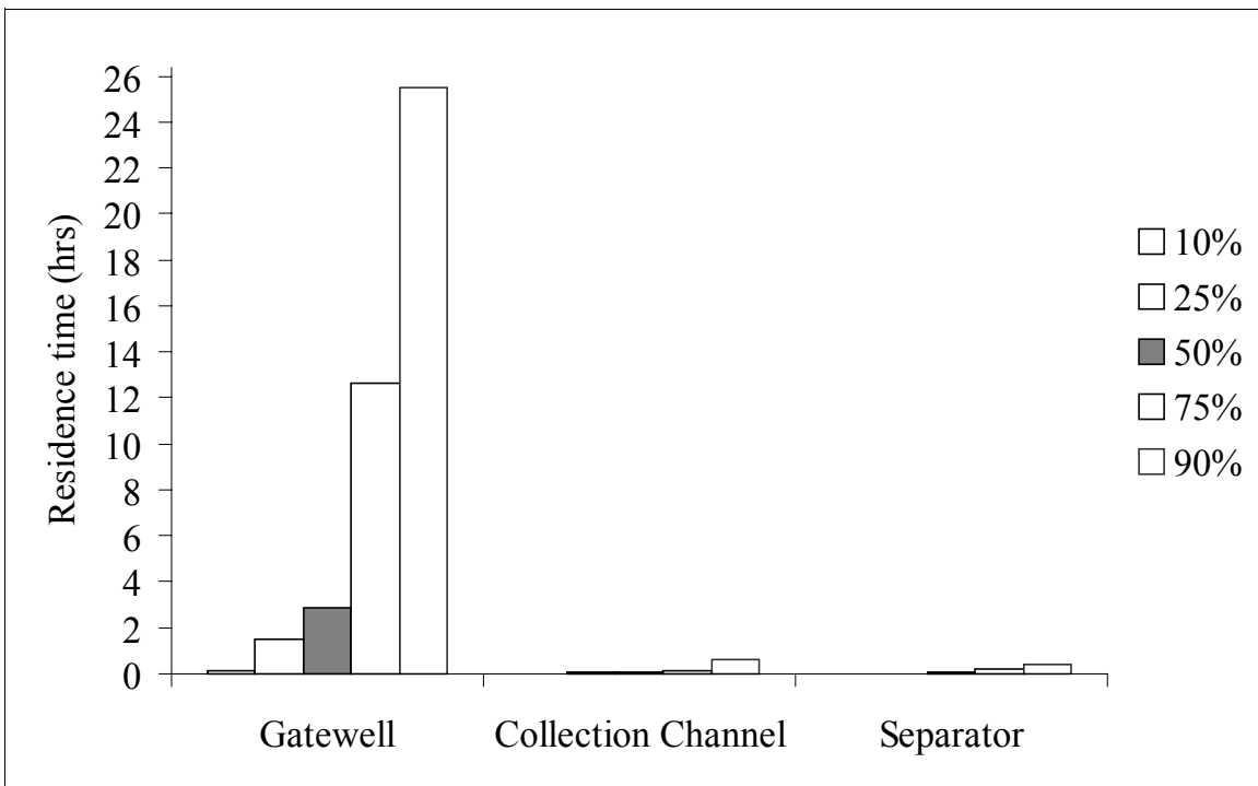
Figure 3. Gatewell, collection channel, and separator residence times for percentiles of fish passage at McNary Dam, 2000.
