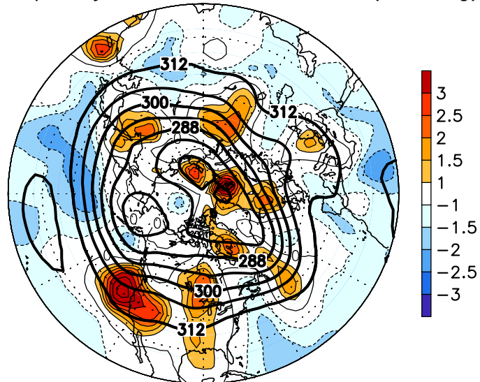
FIGURE E13. Northern Hemisphere: 700-hPa heights for OCT 2007 overlaid with standard deviation of high-pass filtered height (left) and normalized anomalous variance of high-pass filtered height (right). Heights are indicated by thick solid contours in both panels (interval is 60 m). High-pass filtered fields reflect fluctuations having periods less than 10 days, and are indicated by thin contours and shading. Contour interval for standard deviation is 15 m with values > 45 m shaded. Contour interval for normalized variance is 1 standard deviation, with positive values shown by solid contours and dark shading and negative values shown by dashed contours and light shading. Anomalies are departures from the 1964-93 base period monthly means.
