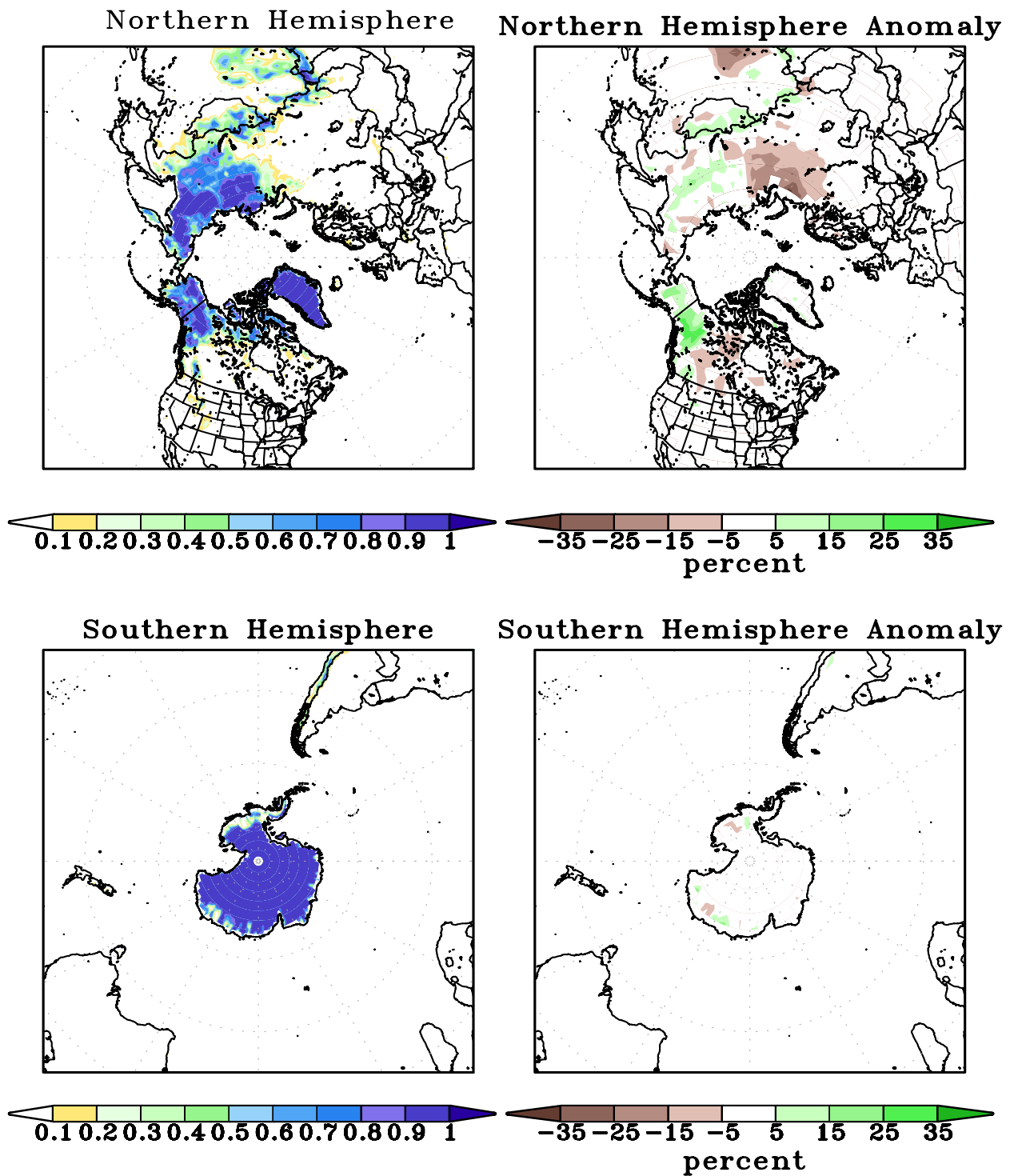
FIGURE A2.2. SSM/I derived snow cover frequency (%) (left) and snow cover anomaly (%) (right) for the month of OCT 2007 based on 1987 - 2006 base period for the Northern Hemisphere (top) and Southern Hemisphere (bottom). It is generated using the algorithm described by Ferraro et. al, 1996, Bull. Amer. Meteor. Soc., vol 77, 891-905.
