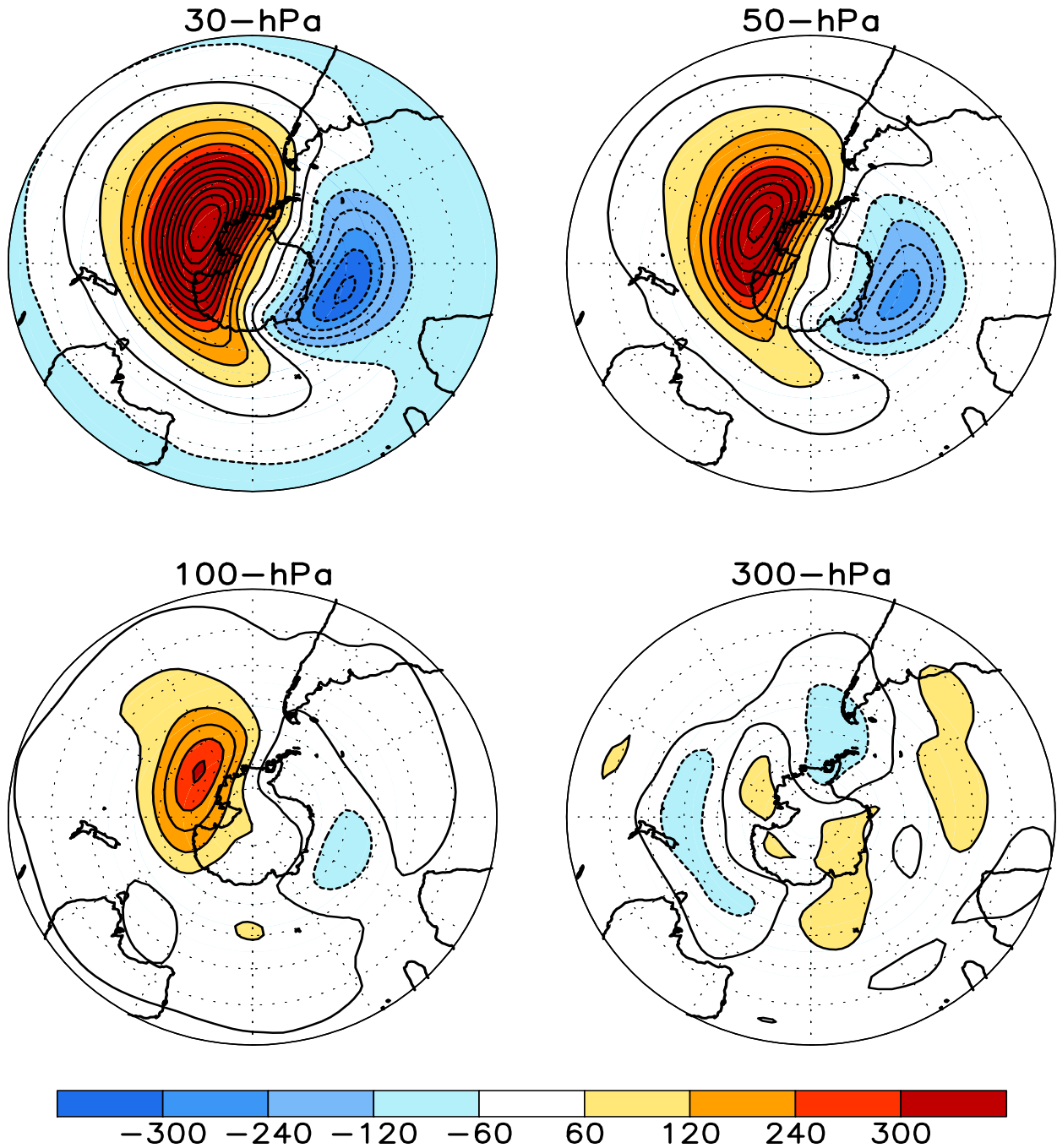
FIGURE S1. Stratospheric height anomalies (m) at selected levels for OCT 2007. Positive values are indicated by solid contours and dark shading. Negative values are indicated by dashed contours and light shading. Contour interval is 60 m. Anomalies are calculated from the 1979–95 base period means. Winter Hemisphere is shown.
