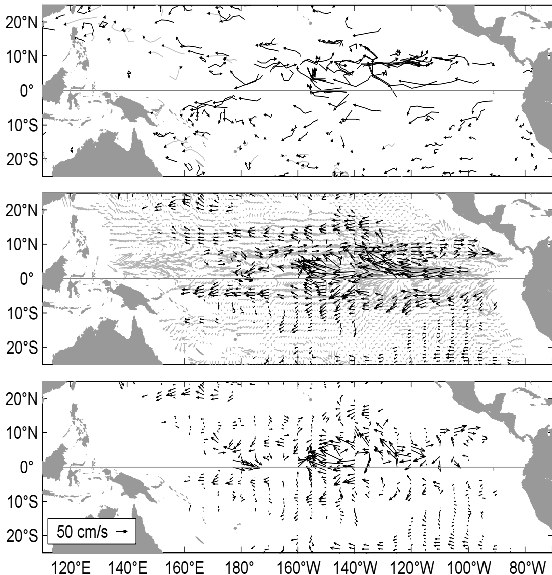
Figure A1.1 Top: Movements of drifting buoys in the tropical Pacific Ocean during October 2007. The linear segments of each trajectory represent a one week displacement. Trajectories of buoys which have lost their subsurface drogues are gray; those with drogues are black.
