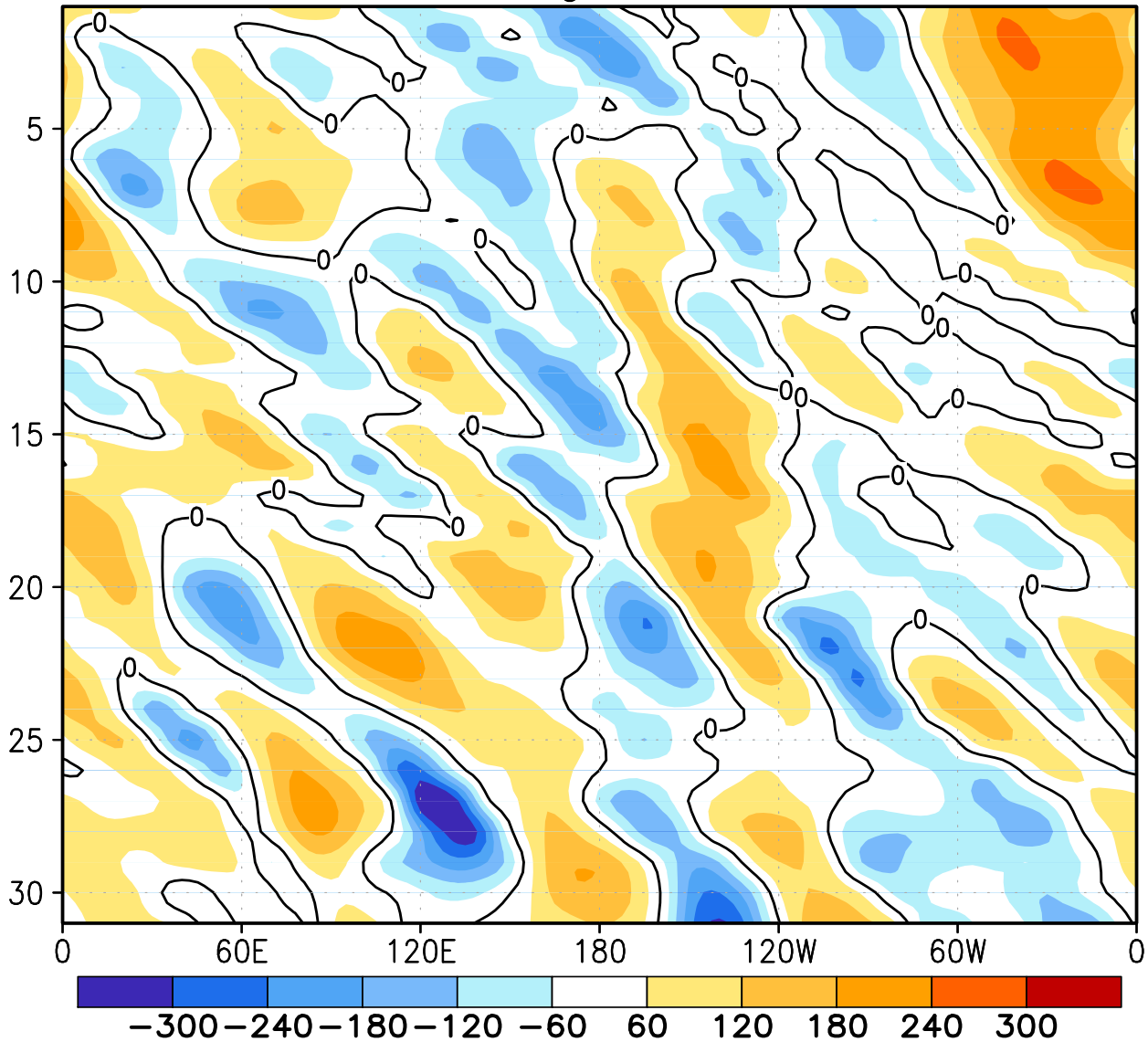
FIGURE E18. Southern Hemisphere: Daily 500-hPa height anomalies for OCT 2007 averaged over the 5° latitude band centered on 40°S. Positive values are indicated by solid contours and dark shading. Negative values are indicated by dashed contours and light shading. Contour interval is 60 m. Anomalies are departures from the 1979-95 base period daily means.
