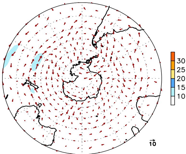
FIGURE E16. Southern Hemisphere mean (left) and anomalous (right) 300-hPa vector wind (CDAS/Reanalysis) for OCT 2007. Mean (anomaly) isotach contour interval is 10 (5) \text{ms}^{-1} . Values greater than 30 \text{ms}^{-1} (left) and 10 \text{ms}^{-1} (rights) are shaded. Anomalies are departures from the 1979-95 base period monthly means.
