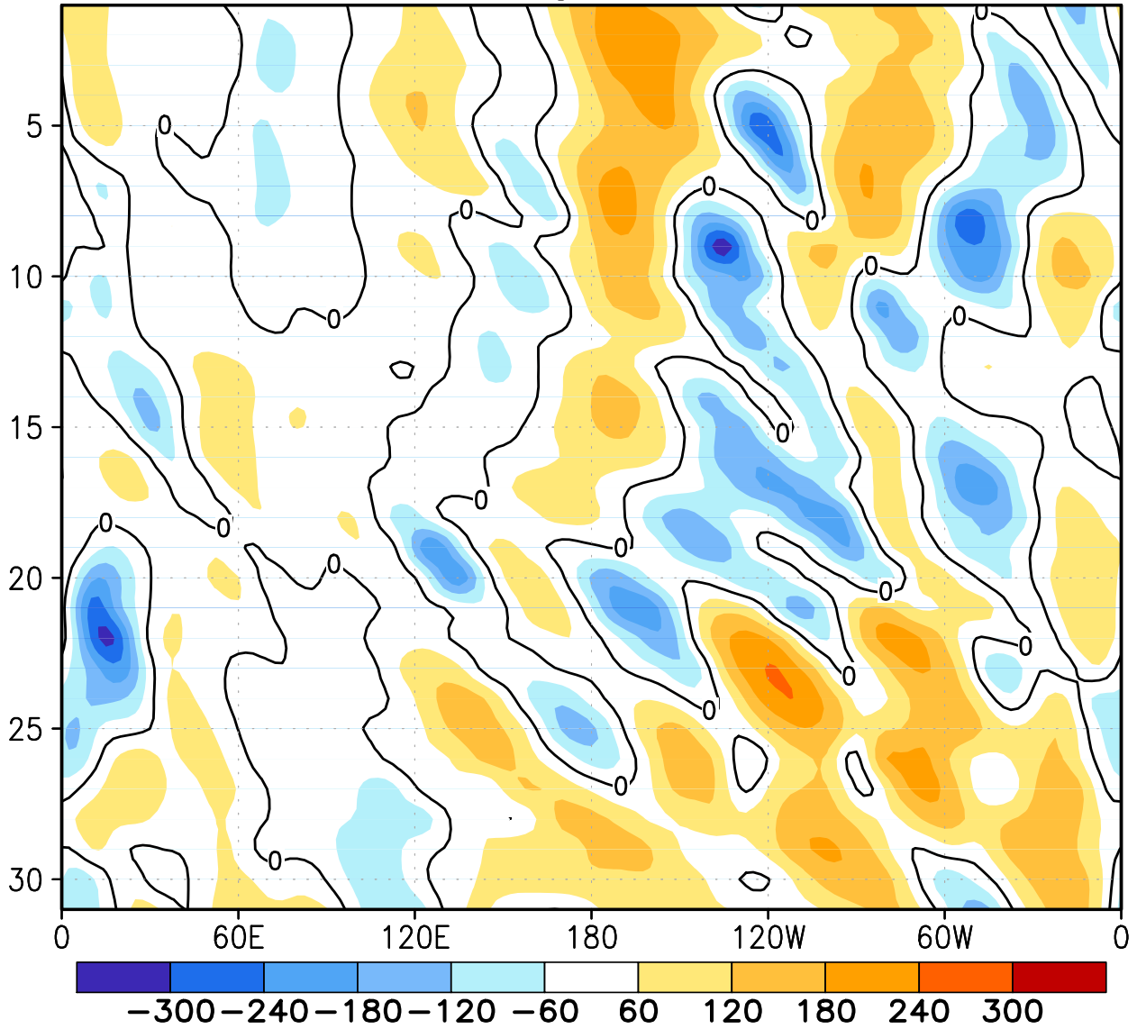
FIGURE E12. Northern Hemisphere: Daily 500-hPa height anomalies for OCT 2007 averaged over the 5° latitude band centered on 40°N. Positive values are indicated by solid contours and dark shading. Negative values are indicated by dashed contours and light shading. Contour interval is 60 m. Anomalies are departures from the 1979-95 base period daily means.
