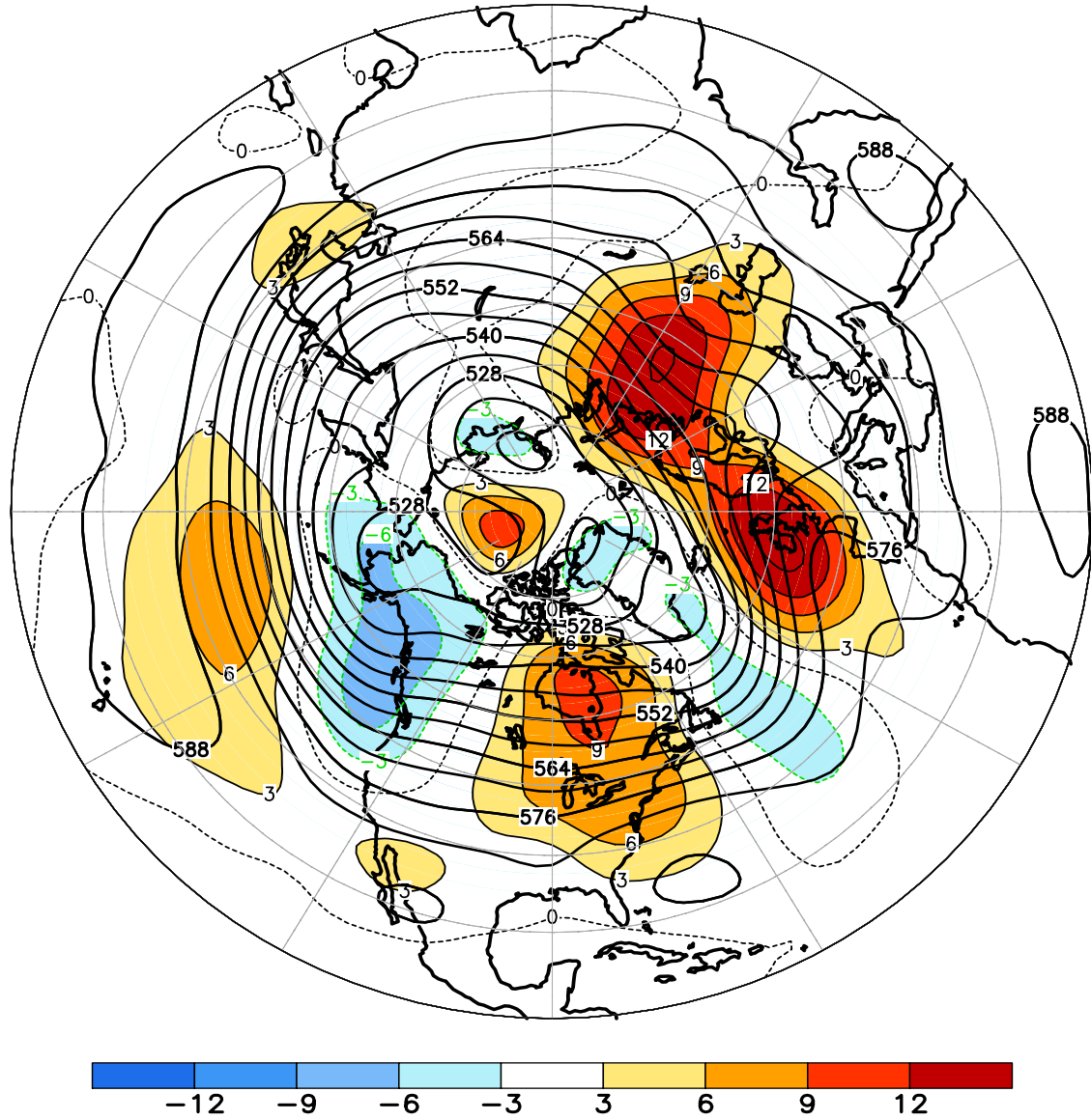
FIGURE E9. Northern Hemisphere mean and anomalous 500-hPa geopotential height (CDAS/Reanalysis) for OCT 2007. Mean heights are denoted by solid contours drawn at an interval of 8 dam. Anomaly contour interval is 3 dam with values less (greater) than -3 dam (3 dam) indicated by dark (light) shading. Anomalies are calculated as departures from the 1979-95 base period monthly means.
