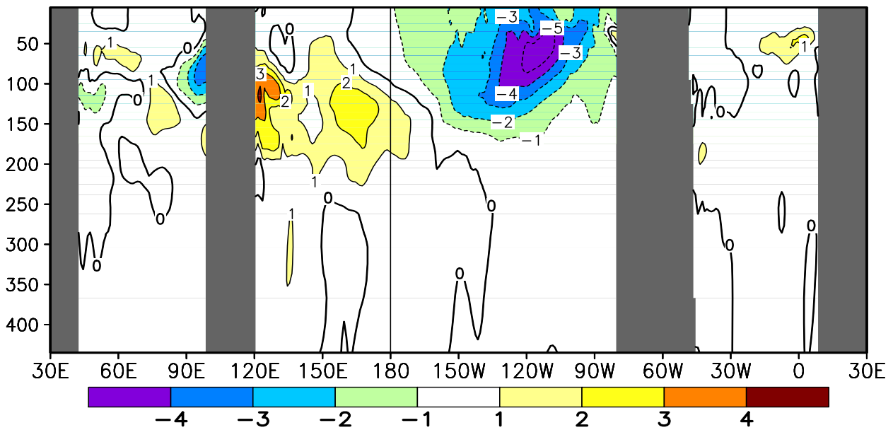
FIGURE T17. Equatorial depth–longitude section of ocean temperature (top) and ocean temperature anomalies (bottom) for OCT 2007. Contour interval is 1°C. Dashed contours in bottom panel indicate negative anomalies. Data are derived from the NCEP’s global ocean data assimilation system version 2 which assimilates oceanic observations into an oceanic GCM (Xue, Y. and Behringer, D.W., 2006: Operational global ocean data assimilation system at NCEP, to be submitted to BAMS). Anomalies are departures from the 1982–2004 base period means.
