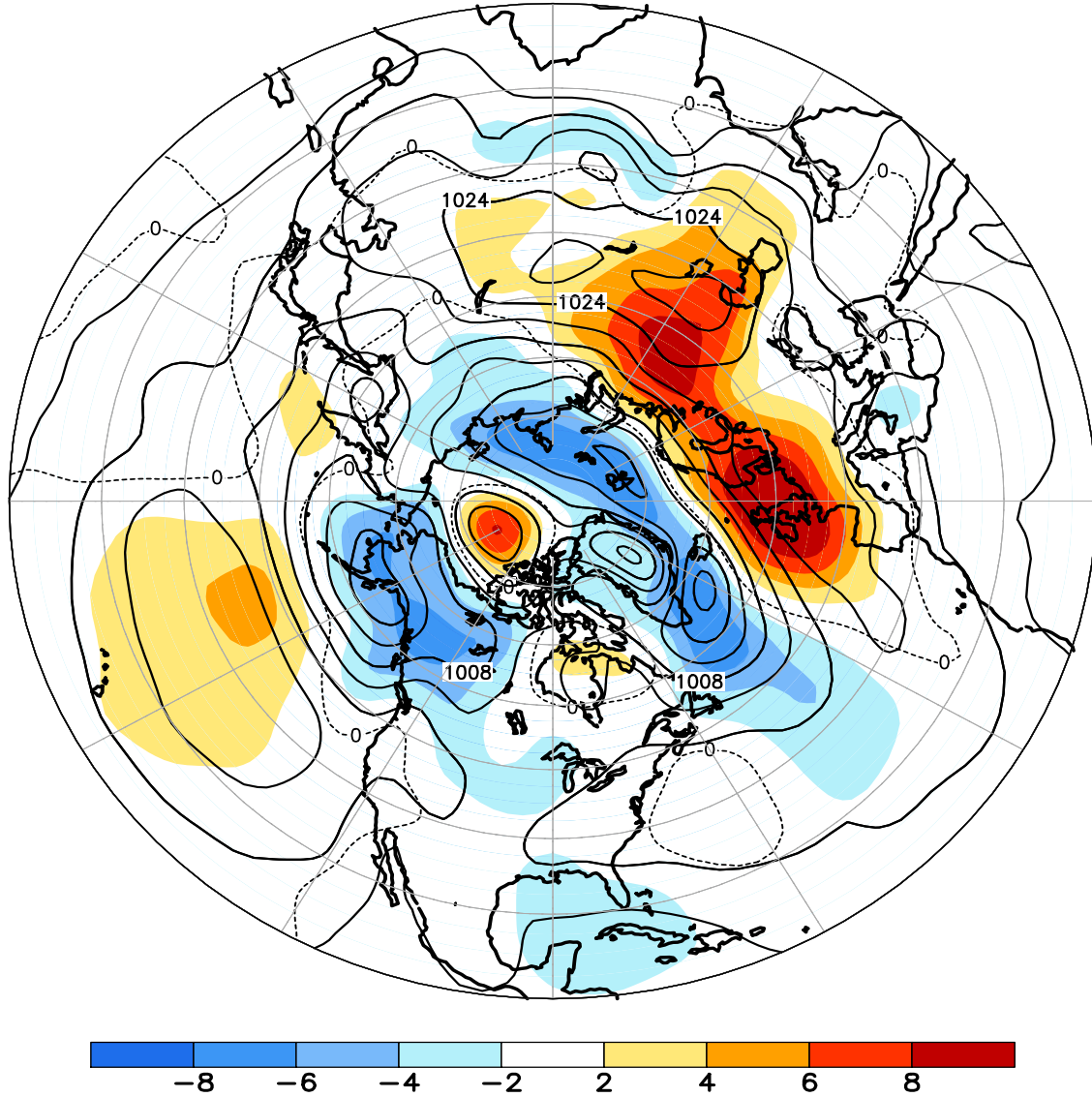
FIGURE E8. Northern Hemisphere mean and anomalous sea level pressure (CDAS/Reanalysis) for OCT 2007. Mean values are denoted by solid contours drawn at an interval of 4 hPa. Anomaly contour interval is 2 hPa with values less (greater) than -2 hPa (2 hPa) indicated by dark (light) shading. Anomalies are calculated as departures from the 1979-95 base period monthly means.
