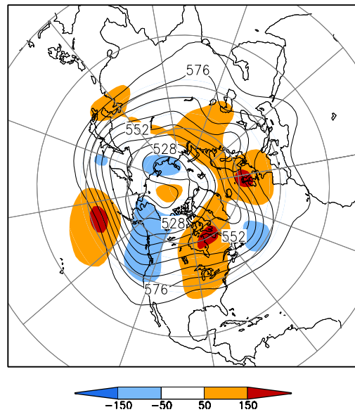
500-hPa Height (dm) & Anomalies (m) (Oct 1–15, 2007)
