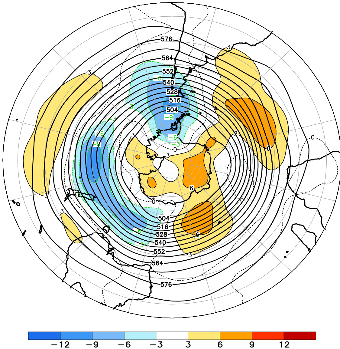
FIGURE E15. Southern Hemisphere mean and anomalous 500-hPa geopotential height (CDAS/Reanalysis) for OCT 2007. Mean heights are denoted by solid contours drawn at an interval of 8 dam. Anomaly contour interval is 3 dam with values less (greater) than -3 dam (3 dam) indicated by dark (light) shading. Anomalies are calculated as departures from the 1979-95 base period monthly means.
