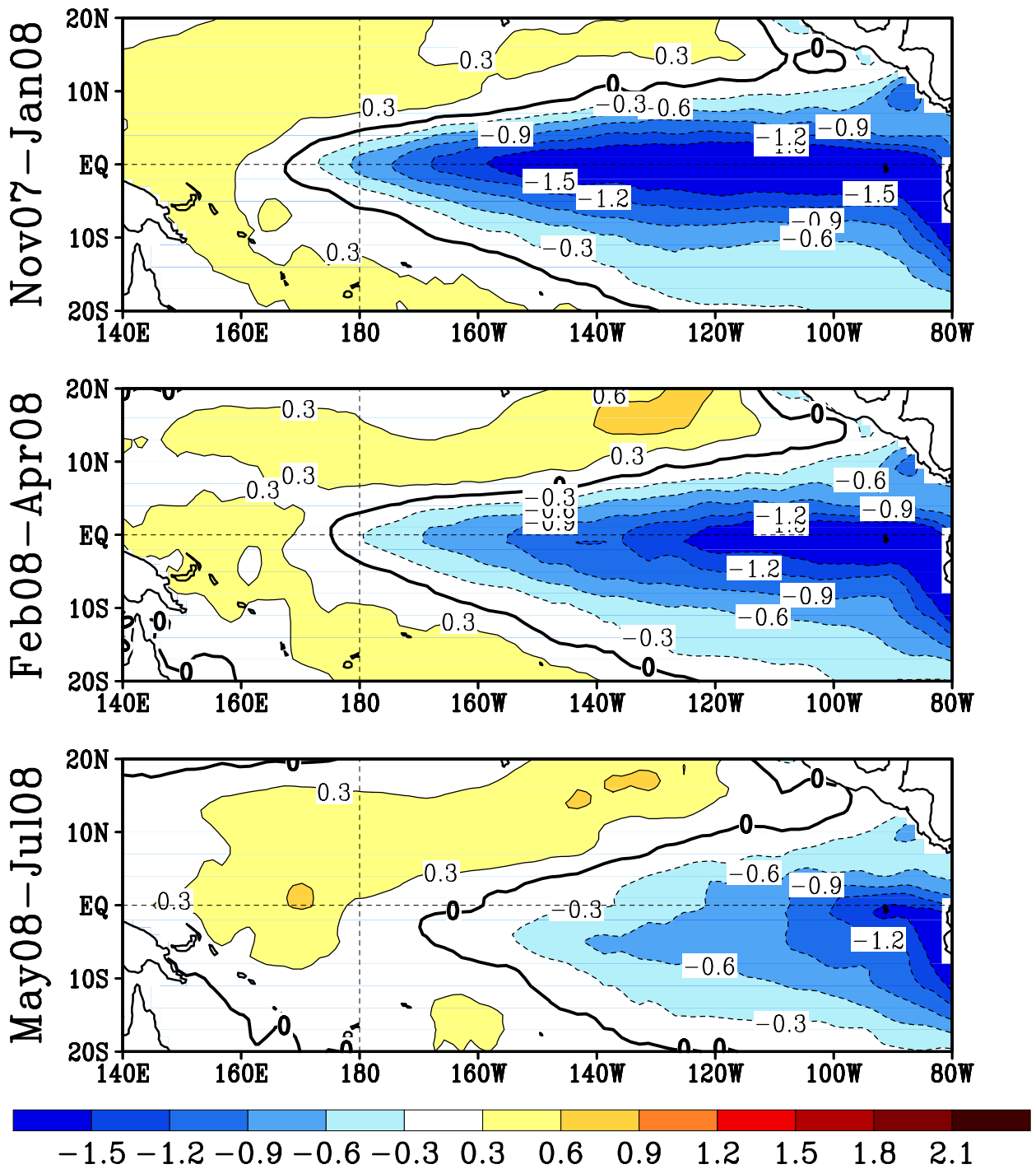
FIGURE F5. Predicted 3-month average sea surface temperature anomalies from the NCEP/CPC Markov model (Xue et al. 2000, J. Climate , 13 , 849-871). The forecast is initiated in OCT 2007 . Contour interval is 0.3C and negative anomalies are indicated by dashed contours. Anomalies are calculated relative to the 1971-2000 climatology.
