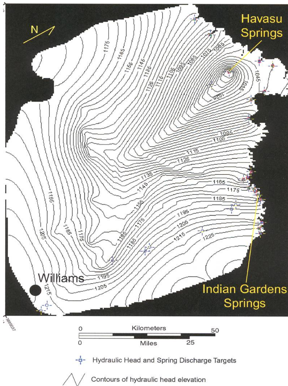
Figure II.4-4. Simulated potentiometric surface in the R-M Aquifer, showing major discharge point at Havasus Springs (after Kessler, 2002).
