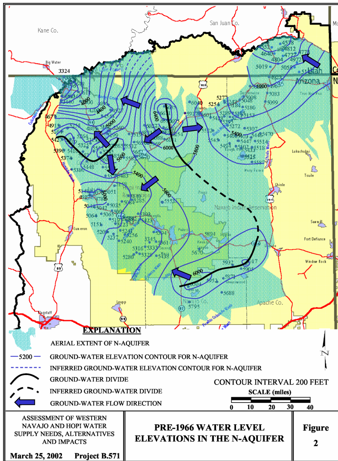
Figure II.4-5. Pre-1996 water level elevations in the N-Aquifer (HDR, 2004).
