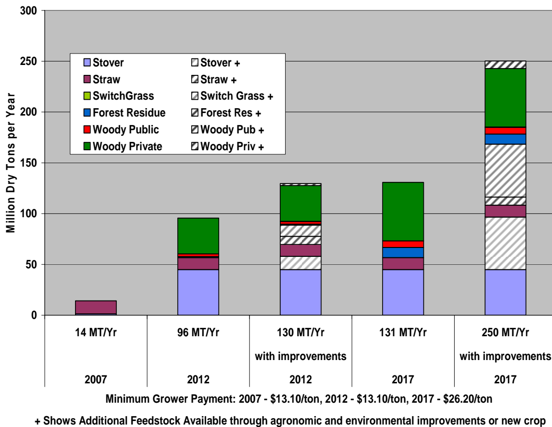
Figure 3-7: Feedstock Available at Specified Minimum Grower Payments
