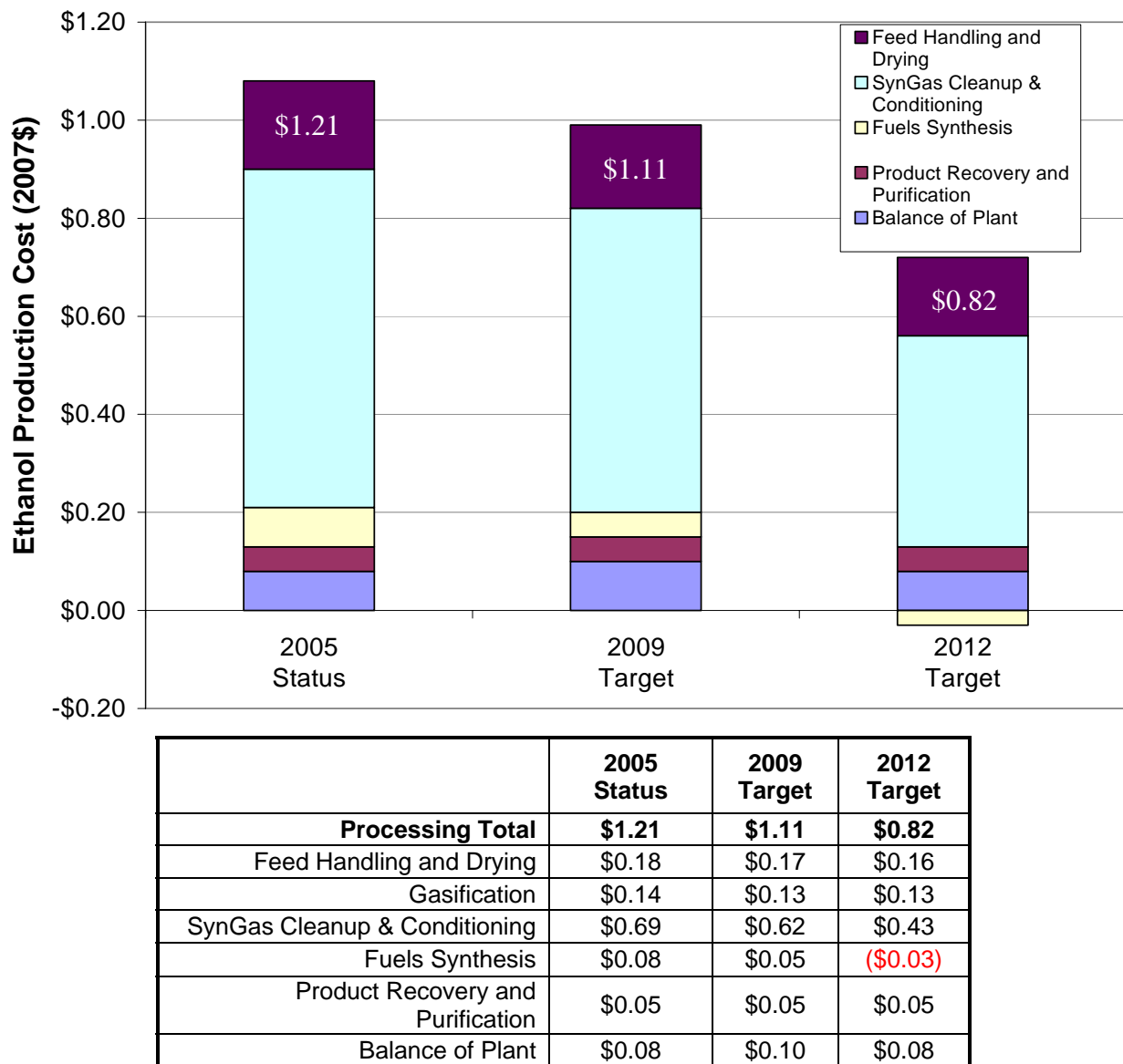
Figure 3-19: Thermochemical Conversion of Hybrid Poplar to Ethanol ($/gal in 2007$)
