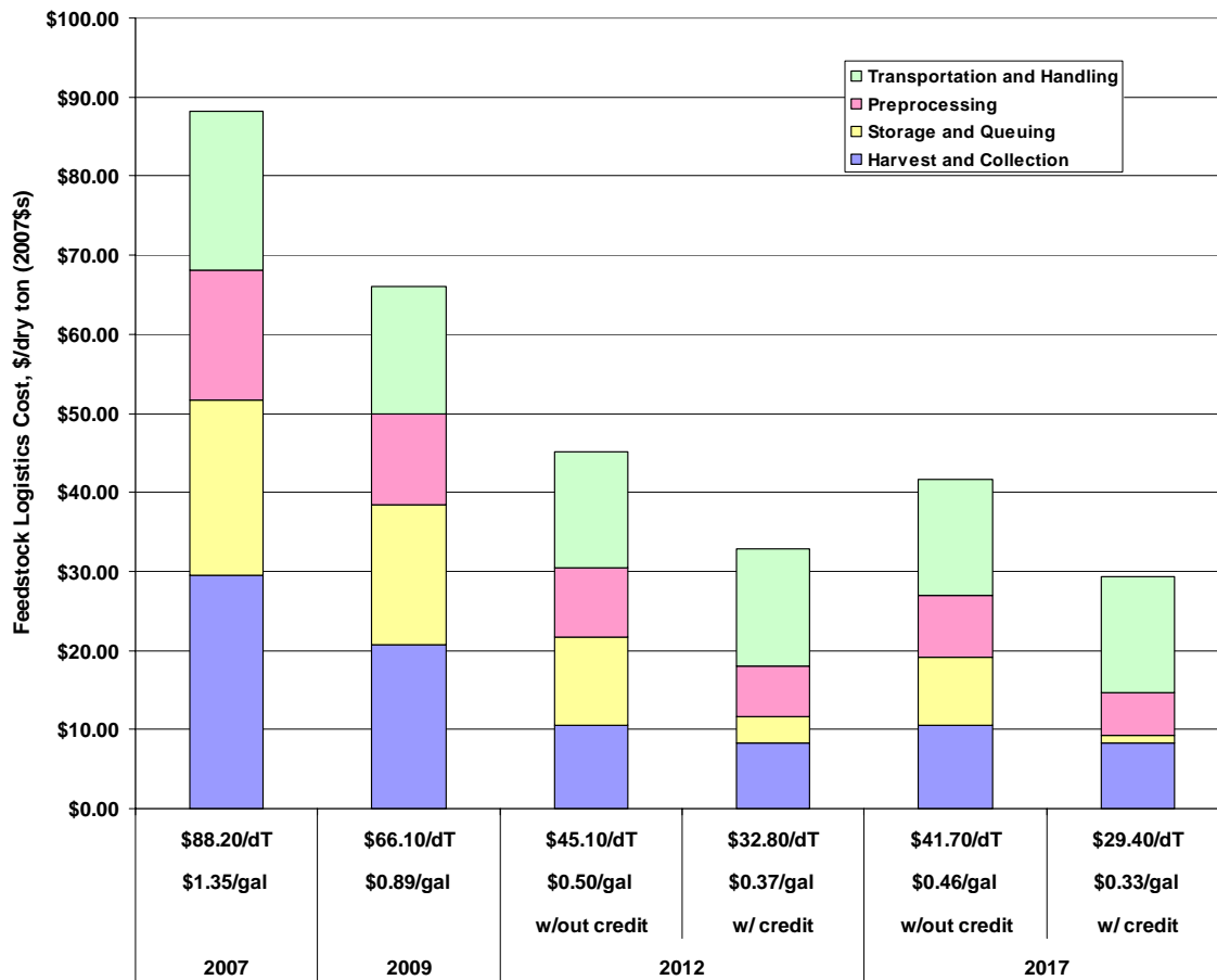
Figure 3-9: Wet Herbaceous Feedstock Logistics Costs
