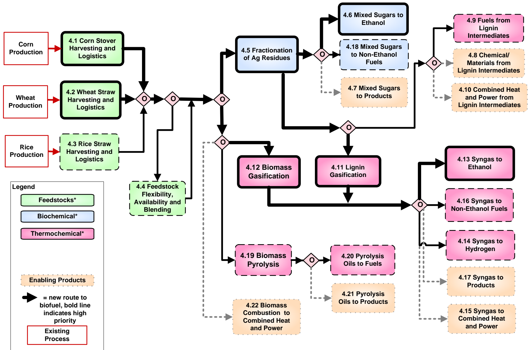
Figure A-4: Agricultural Residue Processing Pathway with Emphasis on Biofuels Routes
