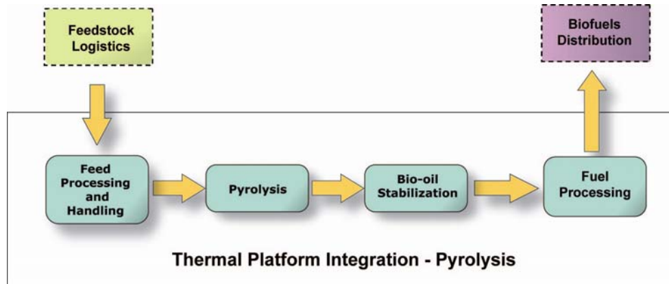
Figure 3-17: Thermochemical Pyrolysis Route for Biomass to Biofuels
