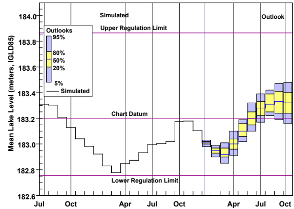
Lake Michigan-Huron Mean Lake Level (meters, IGLD85)
