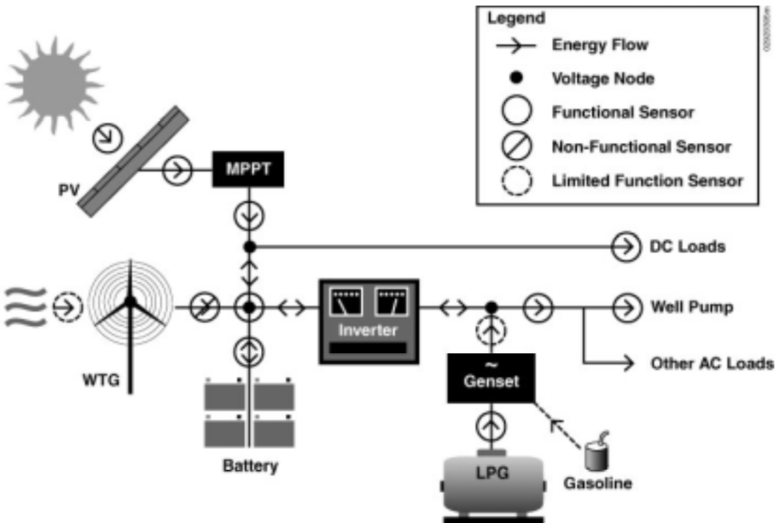
Figure 6.1. Schematic diagram of the electrical system
