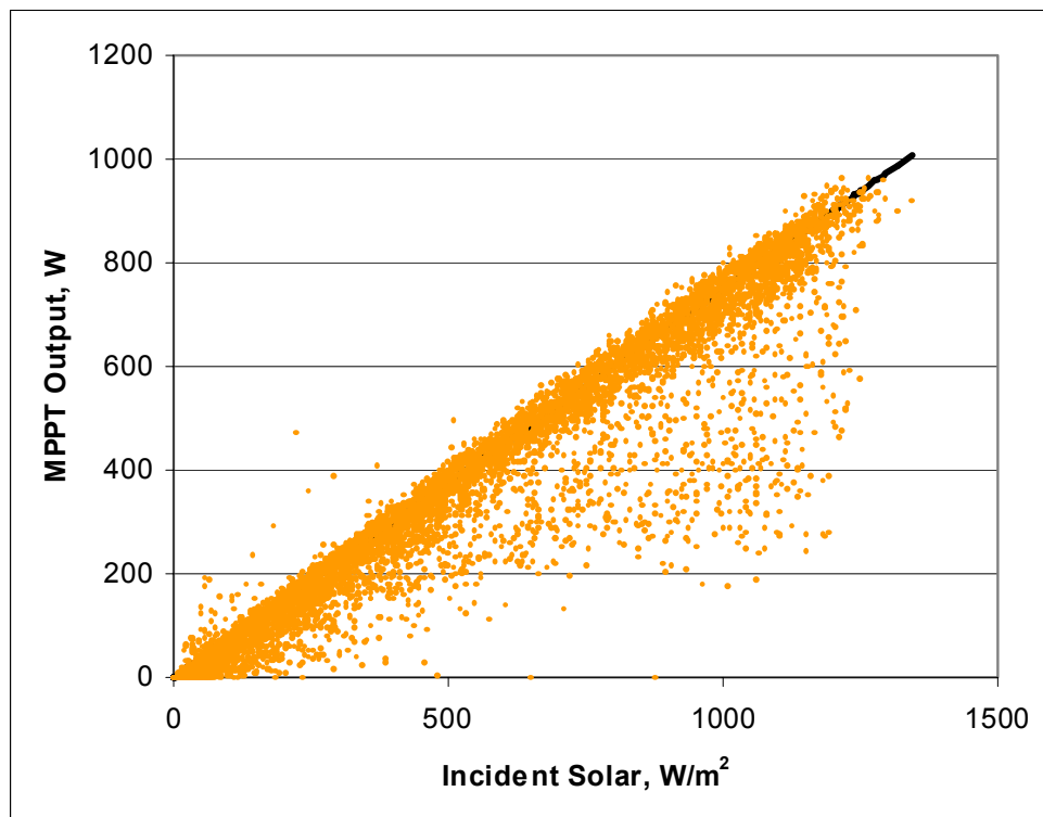
Figure 6.5. Performance of the PV array and MPPT control
