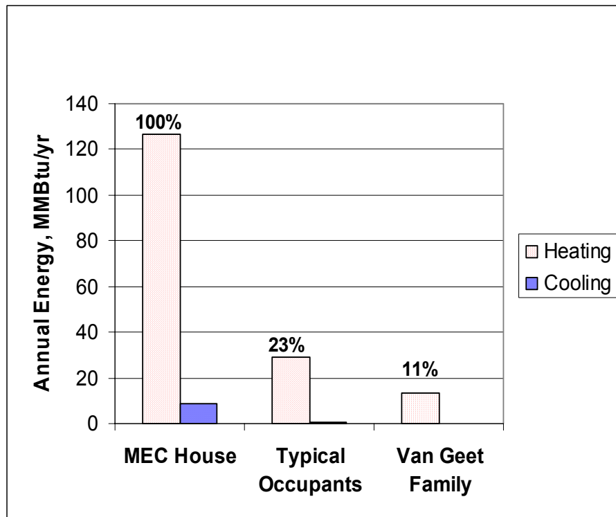
Figure 4.3. Heating and cooling energy savings attributed to house with "typical occupants" and with the Van Geet family's more energy-conservative lifestyle
