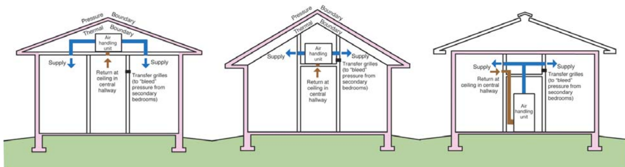
Note: Colored shading depicts the building's thermal barrier and pressure boundary. The thermal barrier and pressure boundary enclose the conditioned space.
