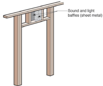
Figure 1-12. Placement of ducts and transfer grilles
