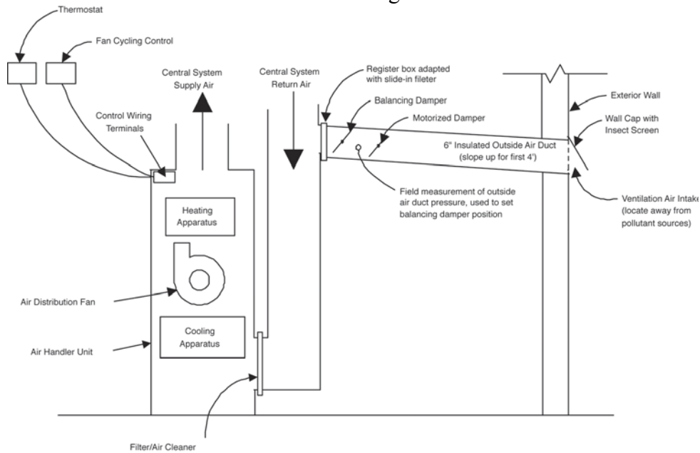
Figure 2-4. Recommended ventilation system in the “Chicago”
