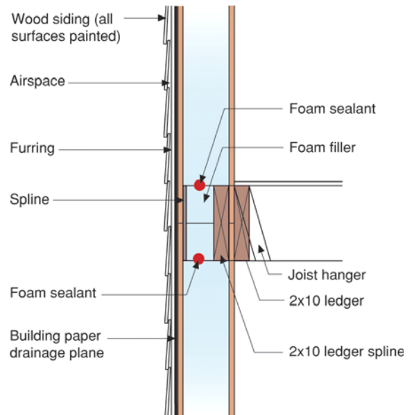
Figure 1-17: Above-grade wall spline
