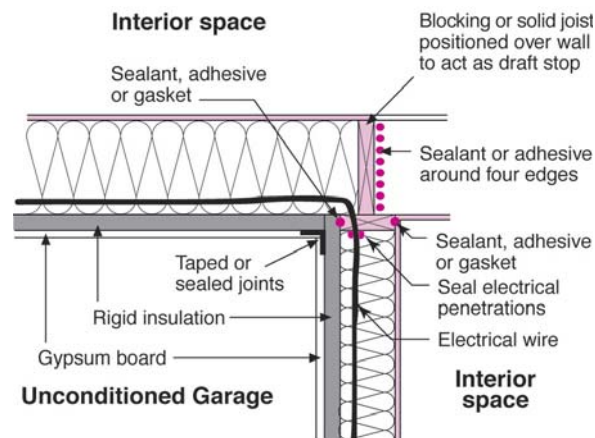
Figure 2-13. Creating a continuous air barrier
