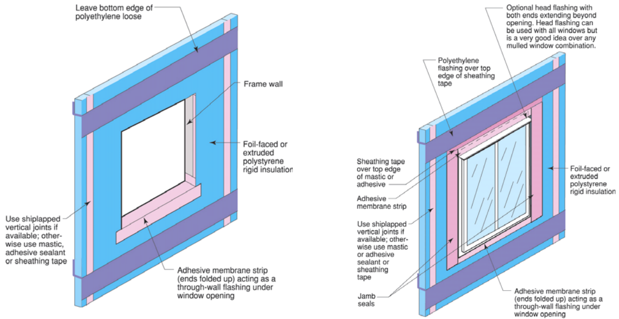
Figure 1-21. Window flashing
