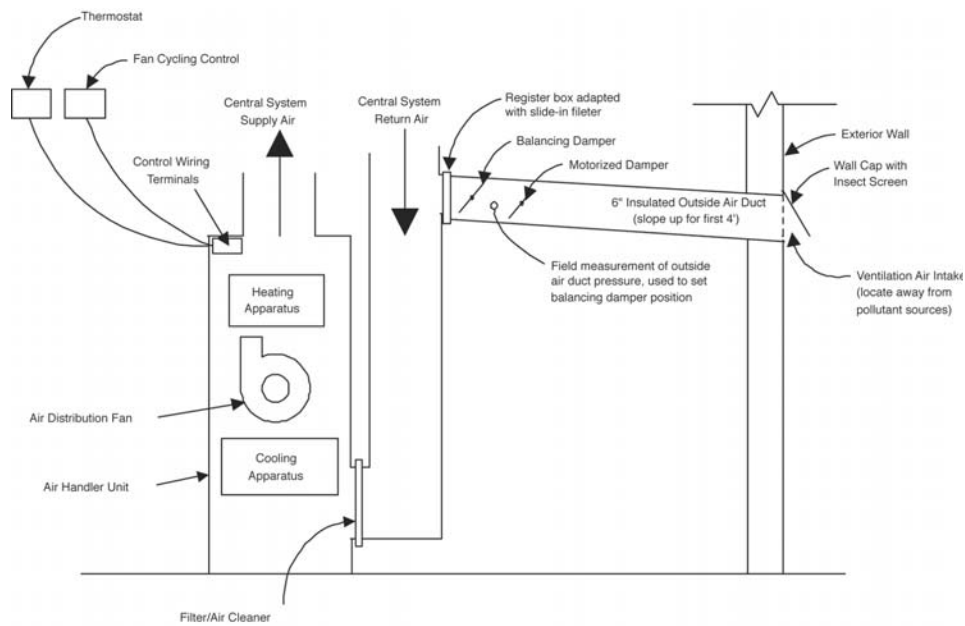
Figure 4-12. HVAC configuration in the “Sacramento”
