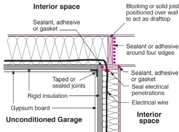
Figure 3-15. Creating a continuous air barrier
