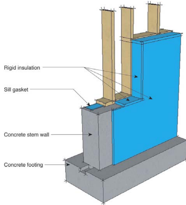
Figure 3-20. Stepped foundation insulation detail
