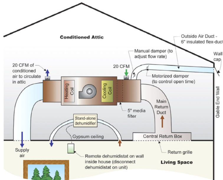
Figure 1-11. Dehumidification
