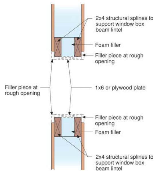
Figure 1-18. Load-bearing window jamb assembly
