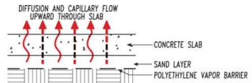
• SAND LAYER BECOMES WATER RESEVOIR TO SUPPLY WATER FOR UPWARD FLOW THROUGH CONCRETE SLAB BY VAPOR DIFFUSION AND CAPILLARY TRANSMISSION • DRYING DOWNWARD BY VAPOR DIFFUSION OR CAPILLARY IS NOT POSSIBLE DUE TO POLYETHYLENE VAPOR BARRIER
