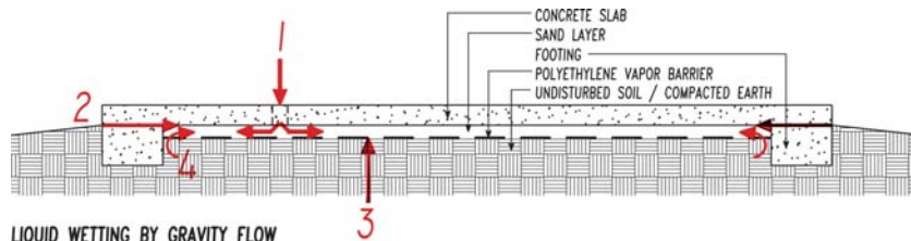
LIQUID WETTING BY GRAVITY FLOW 1. THROUGH TOP OF SLAB BY RAIN, CURING PROCESSES, CUTTING, FINISHING, CLEANING, WATER TESTING, etc. 2. THROUGH SLAB/FOOTING INTERFACE BY IRRIGATION WATER, SURFACE WATER AND GROUND WATER 3. THROUGH JOINTS, PENETRATIONS AND PUNCTURES IN POLYETHYLENE VAPOR BARRIER BY GROUND WATER 4. AROUND THE EDGE OF POLYETHYLENE VAPOR BARRIER AT FOOTING EDGE
