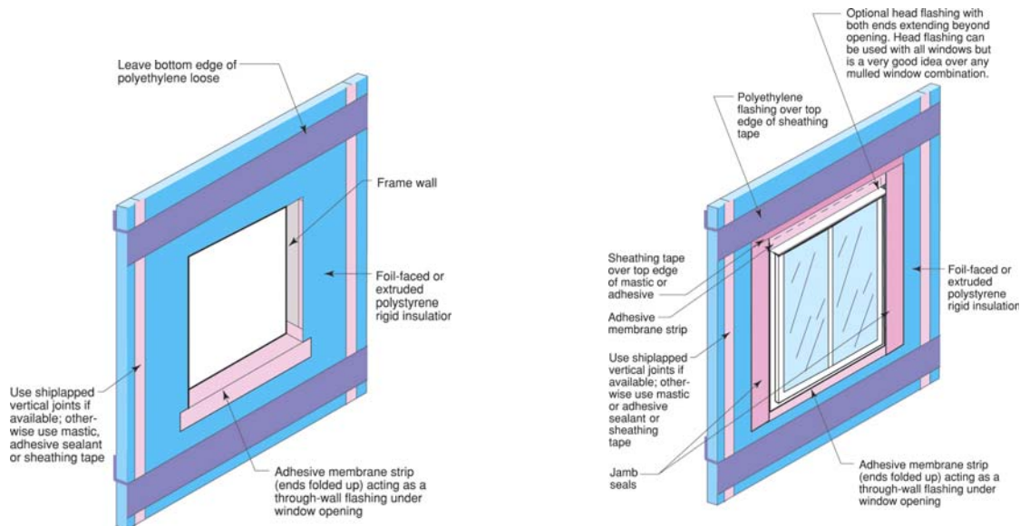
Figure 1-3. Window flashings
