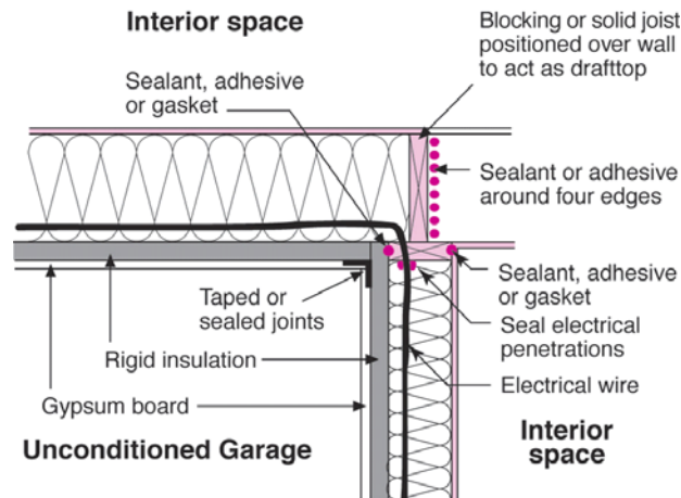
Figure 3-8. Creating a continuous air barrier
