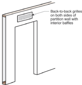
Figure 1-12. Placement of ducts and transfer grilles
