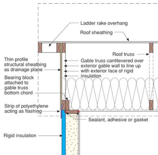
Figure 3-12. Gable end exterior sheathing detail
