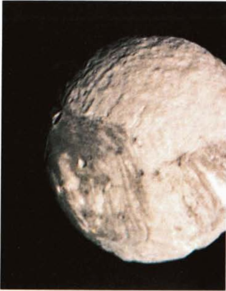
The above is a color composite of the Uranian moon Miranda, taken by Voyager 2 from a distance of 91,000 miles. The picture was constructed from several images acquired by the narrow-angle camera's green, violet and ultra-violet filters. Smallest of Uranus' major satellites, Miranda is more potato-shaped than spherical and has an unusual surface made up of many different geologic forms. The upper right image is a clear-filter closeup of Miranda taken from 26,000 miles; it shows a variety of grooves, ridges and valleys. There are also many impact craters, the largest about 20 miles in diameter, some of the others ranging from three to six miles in diameter. Taken still closer to Miranda, at 22,000 miles, the lower image covers an area about 150 miles across. Two distinct terrain types are visible: the rugged, higher elevation terrain at right and a lower, striated terrain. The big crater in the lower part of the image is estimated at 15 miles in diameter.
