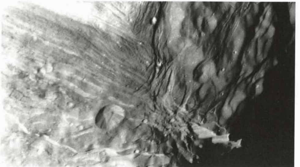
The above is a color composite of the Uranian moon Miranda, taken by Voyager 2 from a distance of 91,000 miles. The picture was constructed from several images acquired by the narrow-angle camera's green, violet and ultra-violet filters. Smallest of Uranus' major satellites, Miranda is more potato-shaped than spherical and has an unusual surface made up of many different geologic forms. The upper right image is a clear-filter closeup of Miranda taken from 26,000 miles; it shows a variety of grooves, ridges and valleys. There are also many impact craters, the largest about 20 miles in diameter, some of the others ranging from three to six miles in diameter. Taken still closer to Miranda, at 22,000 miles, the lower image covers an area about 150 miles across. Two distinct terrain types are visible: the rugged, higher elevation terrain at right and a lower, striated terrain. The big crater in the lower part of the image is estimated at 15 miles in diameter.
