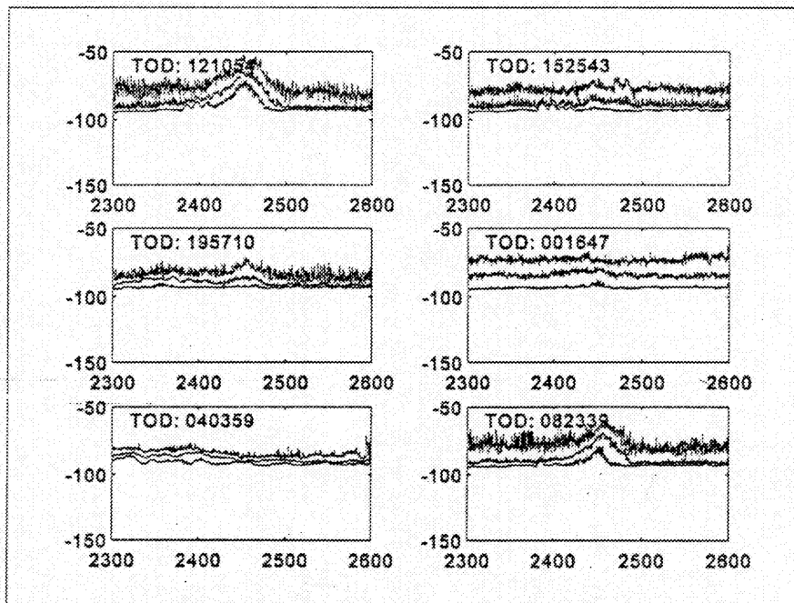
Figure 7: Diurnal Variation in 2300-2600 MHz Spectral Usage, +Peak Mode, 3 MHz Receiver BW, Downtown Denver CO Data, Amplitude(dBm) vs Frequency(MHz).
