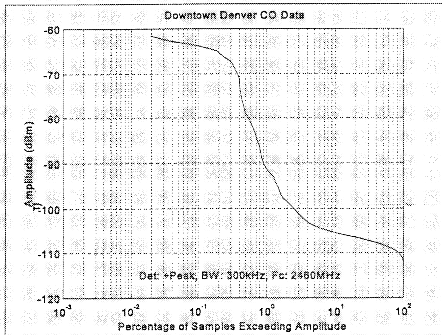
Figure 15: Example of "Dominant Oven" Effect on Signal Amplitude Probability Distribution
