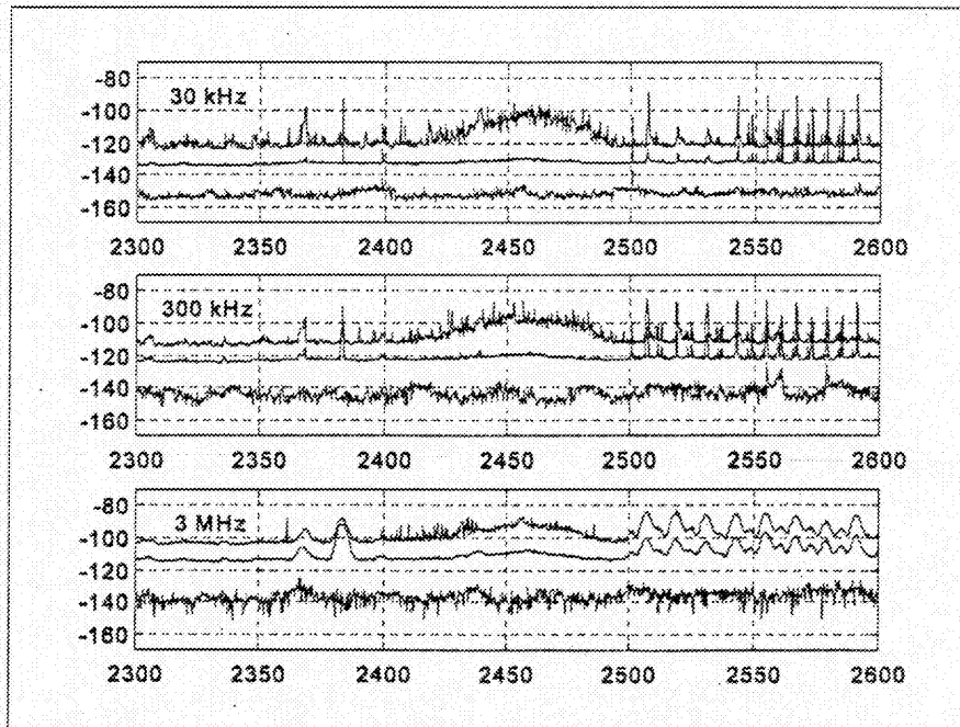
Figure 13: Cumulative Spectral Usage, Sample Mode, Indicated Receiver BW, Los Angeles CA Data, Min of mins, Mean of means, and Max of maxs, Amplitude(dBm) vs Frequency(MHz)
