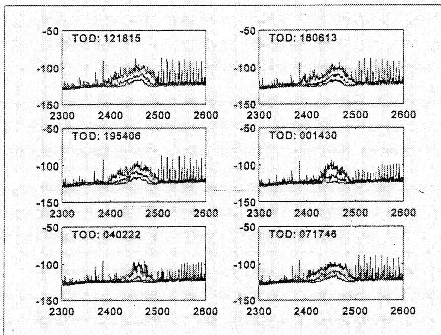
Figure 3: Diurnal Variation in 2300-2600 MHz Spectral Usage, +Peak Mode, 30 kHz Receiver BW, Los Angeles CA data, Amplitude(dBm) vs Frequency(MHz)
