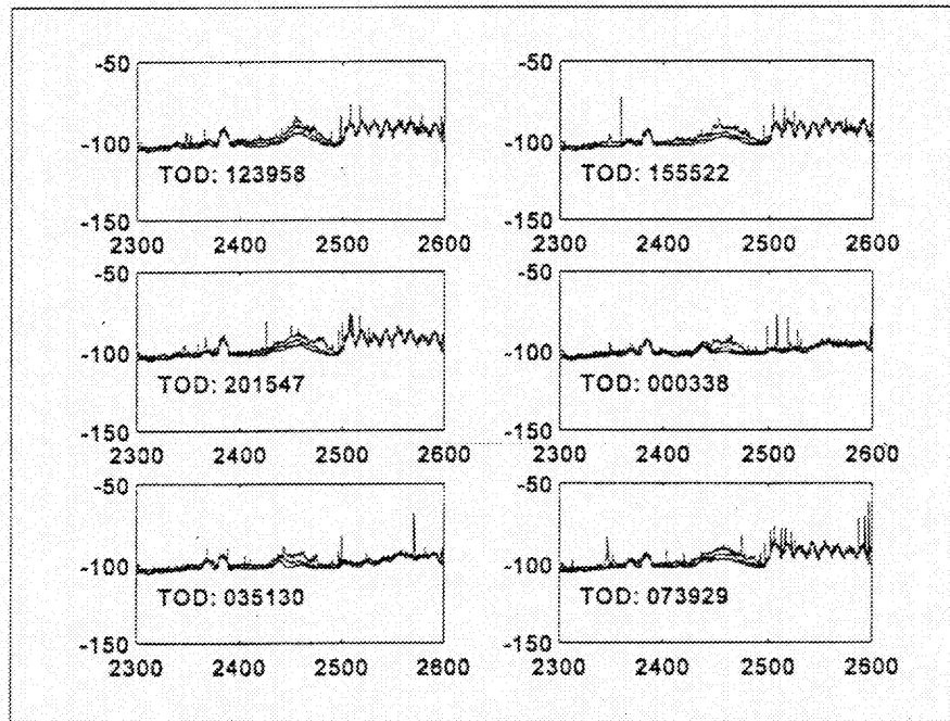
Figure 5: Diurnal Variation in 2300-2600 MHz Spectral Usage, +Peak Mode, 3 MHz Receiver BW, Los Angeles CA Data, Amplitude(dBm) vs Frequency(MHz)
