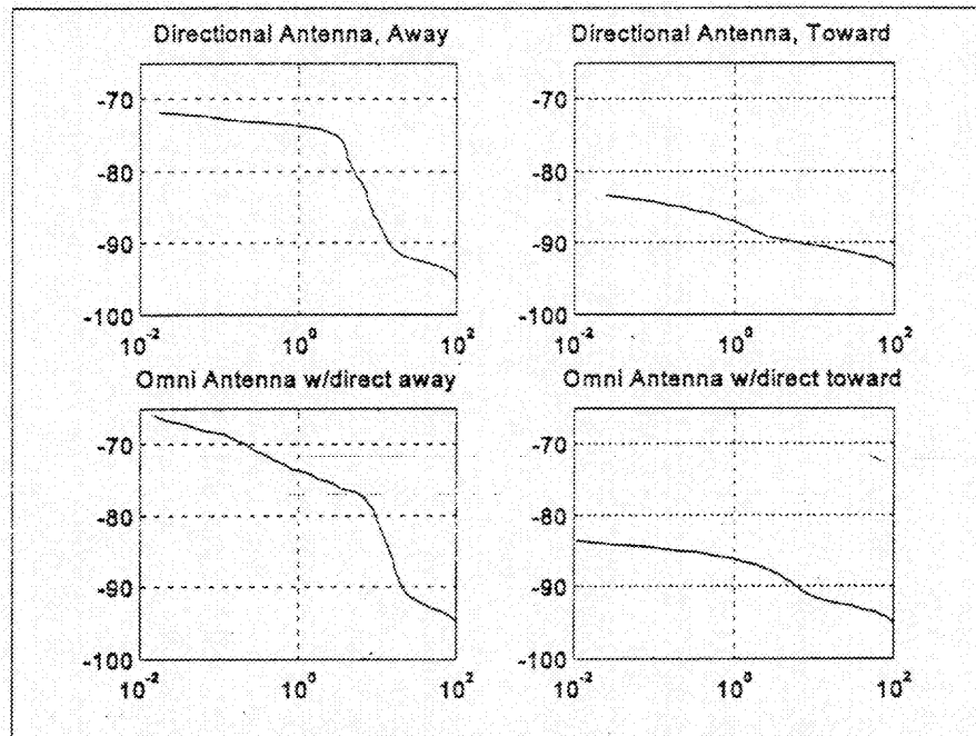
Figure 17: Downtown Denver CO Data, 2450 MHz, +Peak Mode, 3 MHz Receiver BW, Amplitude(dBm) vs Percentage of Samples Exceeding that Amplitude
