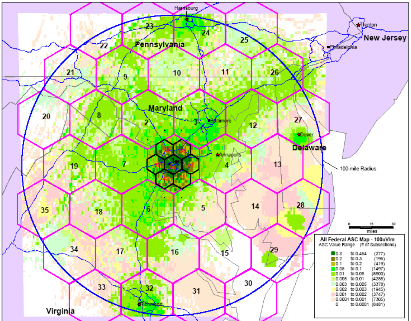
Figure 3-3. Large-Small-Service-Area-Overlapping System Architecture Map
