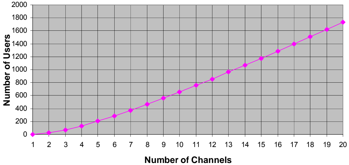
Figure A-1. Trunked Radio Network Dimensioning
