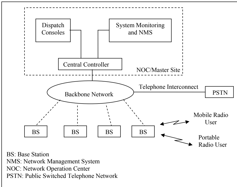
Figure 2-1. Typical Configuration of a Trunked Radio System
