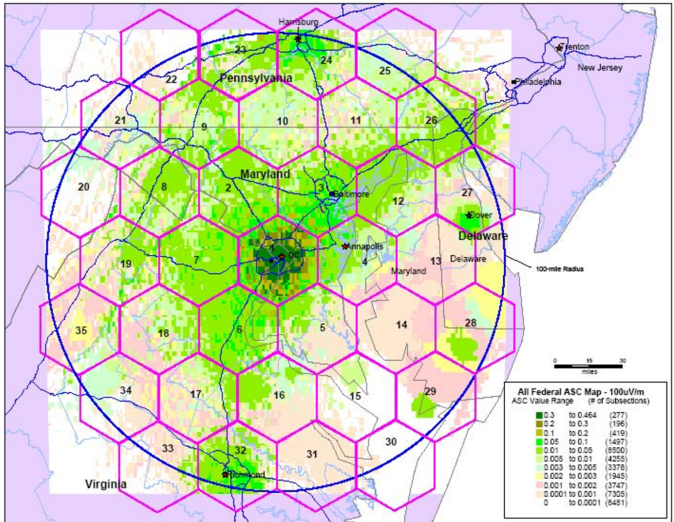
Figure 3-1. Large-Service-Area-Only System Architecture Map
