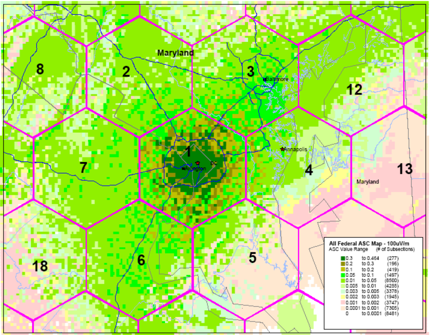
Figure 2-3. Example of ASC Map with Hexagon Service Areas Overlaid
