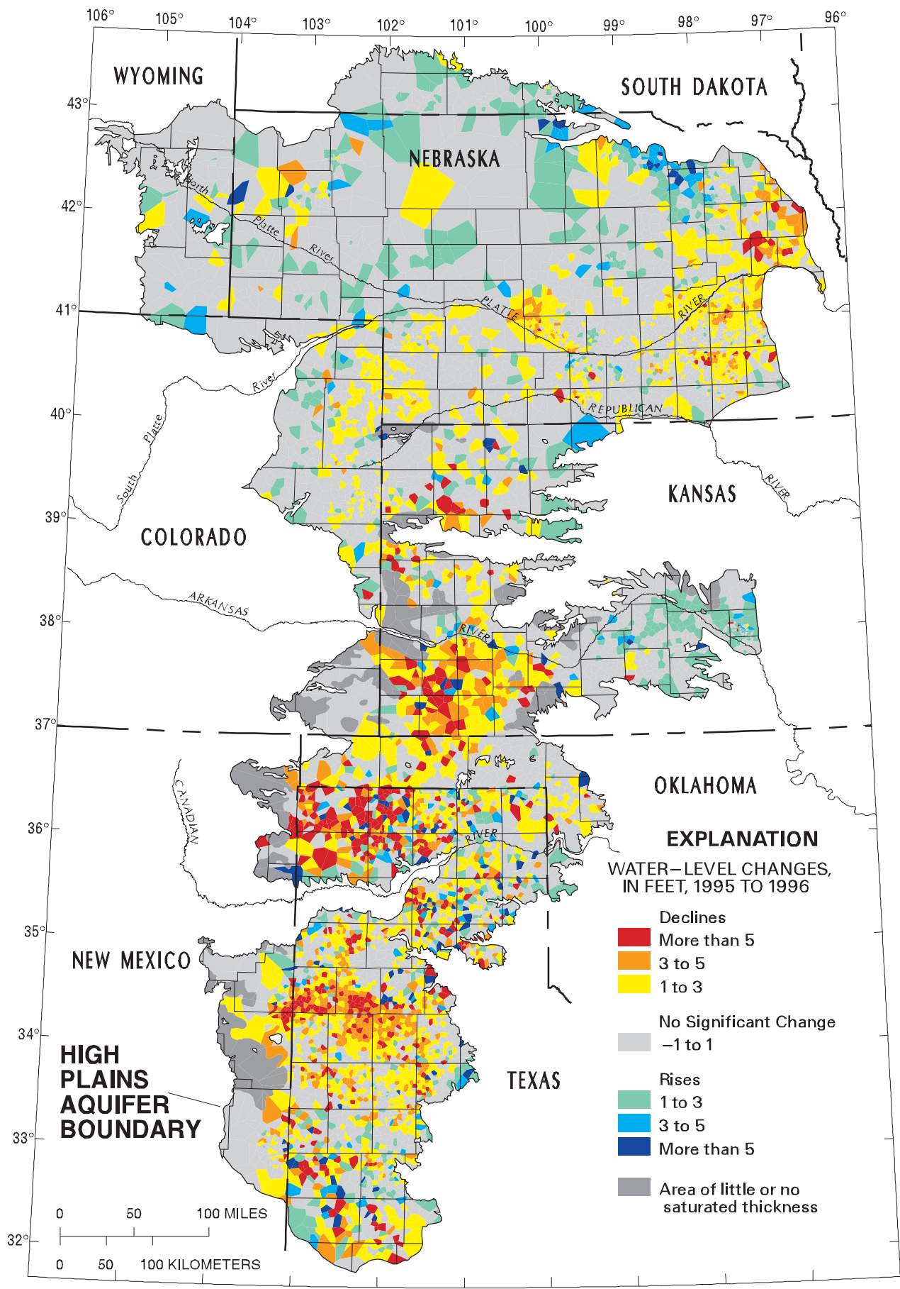
Figure 3. Water-level changes in the High Plains aquifer. 1995 to 1996.
