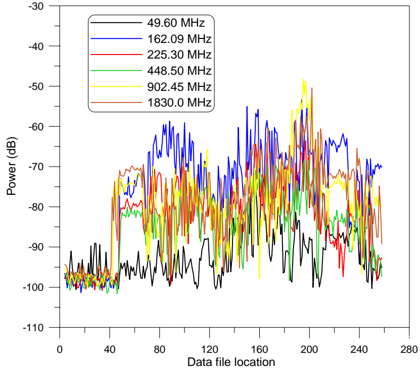
Figure 38. Signal strength measurements around the perimeter of the stadium for the transmitters located at fixed Site B and vertically polarized receiving antennas.
