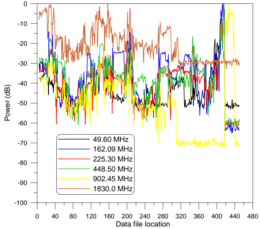
Figure 28. Stadium walk-through for horizontally polarized receiving antennas (playing field).
