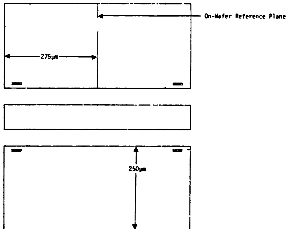
Figure 3. The thru line standard is shown. The on-wafer reference plane is placed exactly in the center of the thru line structure.
