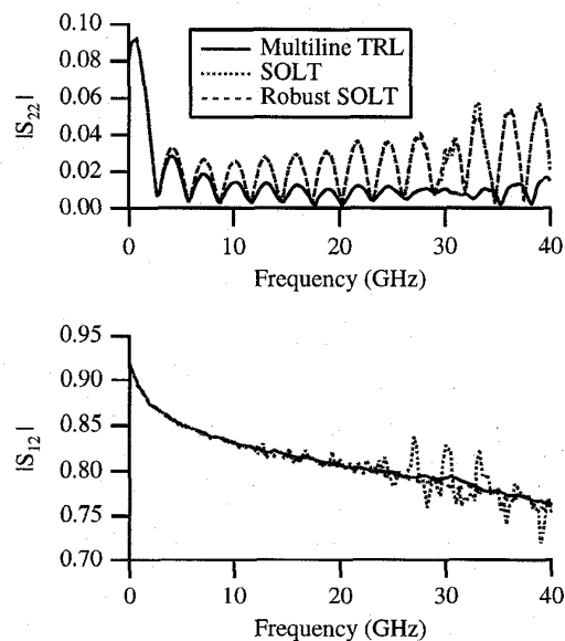
Fig. 3. Magnitude of S_{22} and S_{12} using Multiline TRL, SOLT, and Robust SOLT to measure a 19 mm coplanar waveguide transmission line. The open standard is defined by the simplest model. S_{11} and S_{21} are nearly identical to S_{22} and S_{12} , respectively.
